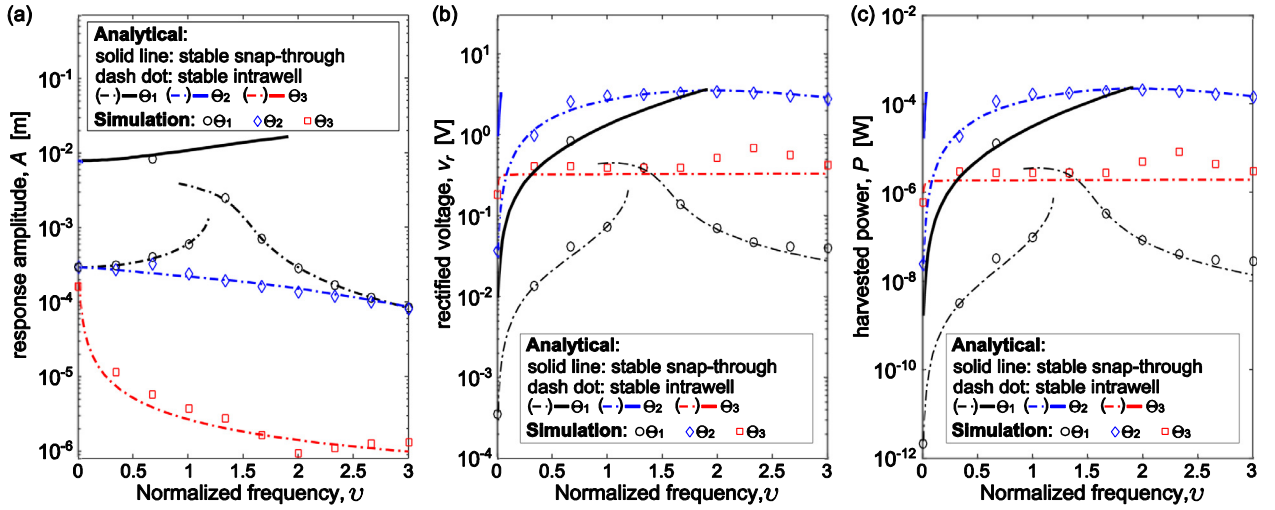
Fig. 13. Influence of coupling constants on (a) dynamic response, (b) rectified voltage and (c) harvested power. The excitation level is p = 7 \text{ m/s}^2 and the coupling constants are set to be \Theta_1 = 3.27 \times 10^{-5} \text{ N/V} ; \Theta_2 = 3.27 \times 10^{-3} \text{ N/V} and \Theta_3 = 3.27 \times 10^{-2} \text{ N/V} .
