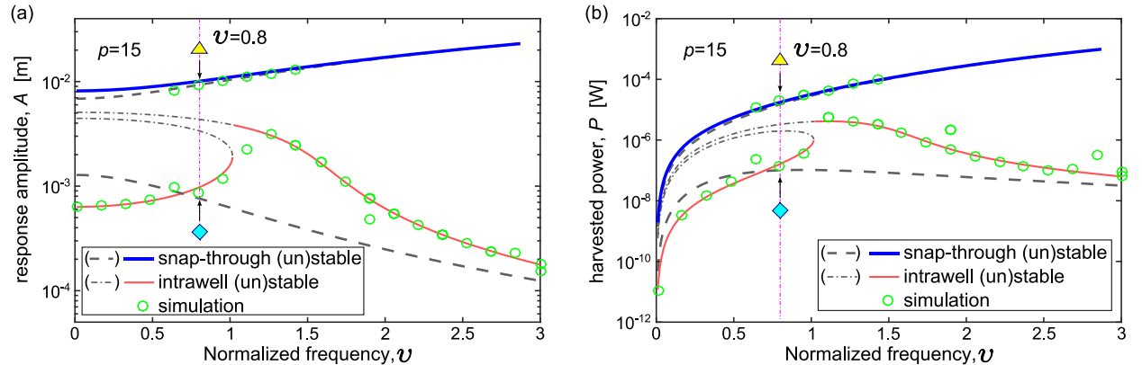
Fig. 6. Frequency dependence of (a) response amplitude and (b) harvested power for p = 15 \text{ m/s}^2 . The triangle and diamond indicate the excitation frequency \nu = 0.8 under which the time varying waveforms of the dynamic responses and induced voltages are numerically estimated and shown in Fig. 7.
