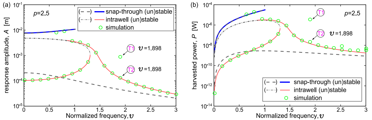
Fig. 5. Frequency dependence of (a) response amplitude and (b) harvested power for p = 2.5 \text{ m/s}^2 .
