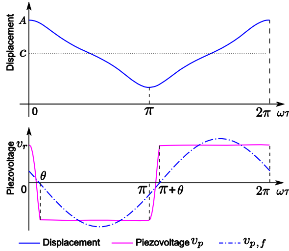
Fig. 2. Typical piezovoltage and its fundamental harmonic component.
