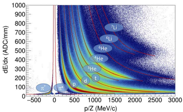
FIG. 20. PID plot for combined ^{132}\text{Sn} + ^{124}\text{Sn} and ^{108}\text{Sn} + ^{112}\text{Sn} systems. Expected PID lines are drawn up to lithium isotopes. The formula converting the ADC channel to Kev is E \text{ (keV)} = 0.00455 * (\text{ADC} + 8.3) .
