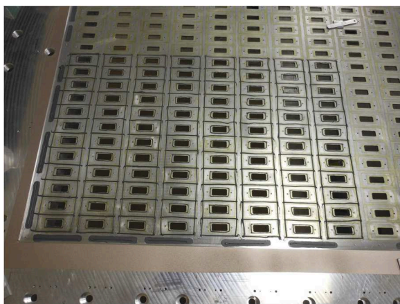
FIG. 8. Photograph of the top plate and glue pattern prior to gluing the pad plane to the top plate. The dark rectangular lines are the Araldite 2013 glue beads.
