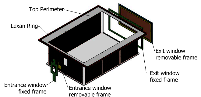
FIG. 9. Schematic view of the field cage. The entrance and exit windows are shown offset from the field cage.
