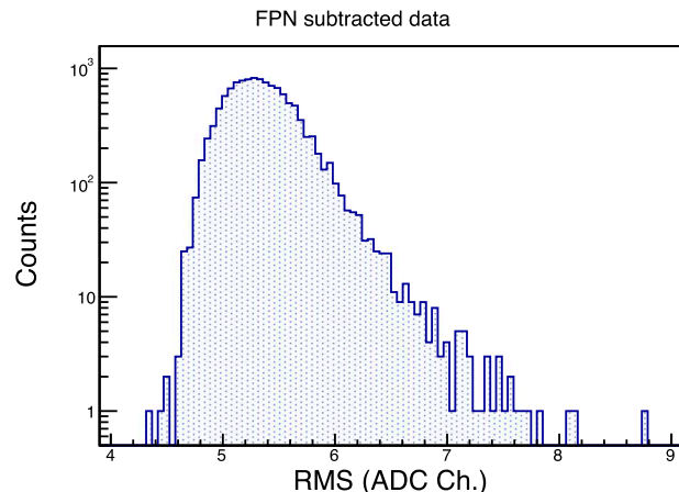
FIG. 5. Distribution of the rms variation of pedestal for all 12 096 ADC channels. Reproduced with permission from G. Jhang, "Performance of the S \pi RIT TPC for the nuclear physics experiment at RIBF," Ph.D. dissertation (Korea University Library, 2016). Licensed under a Creative Commons Attribution (CC BY 2.0) License.
