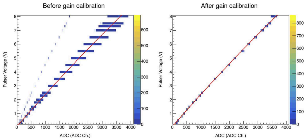
FIG. 6. Distribution of the pad response to pulsed signals on the ground plane before (left) and after (right) performing gain calibration for all 12 096 channels. Reproduced with permission from G. Jhang, “Performance of the S \pi RIT TPC for the nuclear physics experiment at RIBF,” Ph.D. dissertation (Korea University Library, 2016). Licensed under a Creative Commons Attribution (CC BY 2.0) License.
