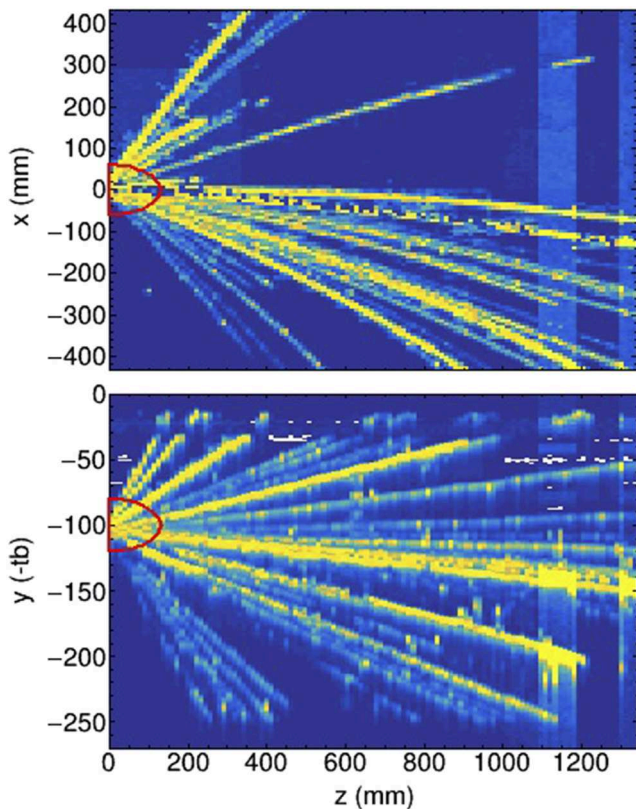
FIG. 19. A typical event in the TPC, shown from (top) above and (bottom) the side. The view from the above corresponds to the pad plane, with each pixel representing a pad, and the side view showing the time measurement, with each pixel representing a pad length and timebucket width.
