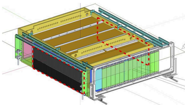
FIG. 15. TPC with the two-panel Kyoto multiplicity array mounted. Only one panel, in black and outlined with the red dashed line, is visible. The other panel is on the opposite side of the TPC, with the outline showing its relative location. Reproduced with permission from Kaneko et al. , RIKEN Accel. Prog. Rep. 50 , 172 (2017). Copyright 2017, RIKEN Nishina Center for Accelerator-Based Science.
