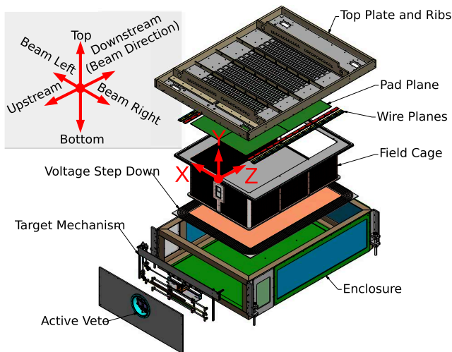
FIG. 2. Exploded view of the SπRIT TPC, with key components labeled and direction indicators in the inset.
