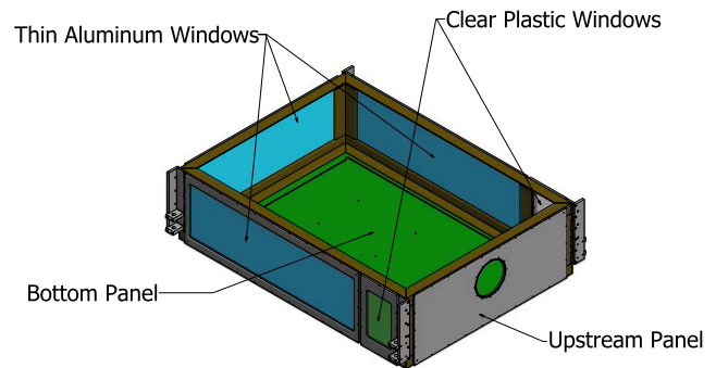
FIG. 13. TPC enclosure design, without the top plate.
