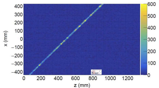
FIG. 16. A cosmic ray recorded in the S\pi RIT TPC pad plane, shown from above.
