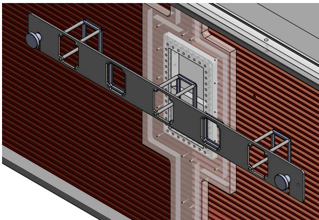
FIG. 12. Location of the target ladder with respect to the field cage.
