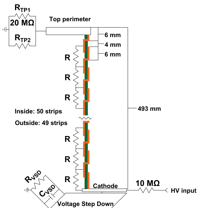
FIG. 10. Schematic view of the field cage resistor chain circuit.
