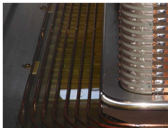
FIG. 11. Field cage and voltage step down.
