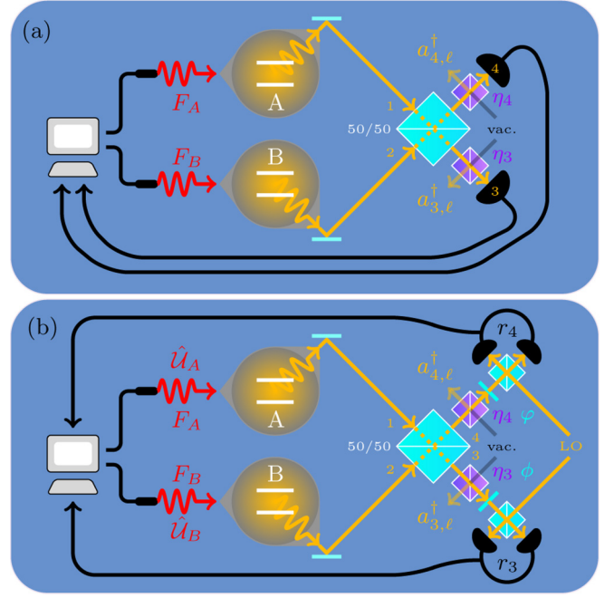
FIG. 1. We illustrate an apparatus for creating and preserving entanglement between qubits A and B, using measurements of spontaneous emission and feedback based on those measurements. Panel (a) shows a device based on photocounting measurements, whereas panel (b) shows a corresponding device based on homodyne detection. In either case, cavities and transmission lines capture spontaneous emission and route it to measurement devices. The emitted signals from each qubit are mixed on a 50:50 beam splitter and then monitored continuously, with a measurement result acquired every integration interval \Delta t . We suppose that \Delta t \ll T_1 . Feedback control is exerted by fast \pi pulses (fast compared to both T_1 and \Delta t ), which quickly flip qubit A ( \hat{F}_A ) and/or qubit B ( \hat{F}_B ). These flips may or may not be implemented at the end of each detector integration time step, conditioned on the measurement outcome. Additional qubit rotations \hat{U}_A and \hat{U}_B are used in the homodyne case (b). The cavities must be engineered such that the photons implementing the \pi pulses, or rotations, do not couple to the output modes which lead to the measurement devices. The purple beam splitters model photon losses, where the incoming signal scatters according to the transformation \hat{a}_i^\dagger \rightarrow \sqrt{\eta_i}\hat{a}_{i,s}^\dagger + \sqrt{1-\eta_i}\hat{a}_{i,\ell}^\dagger ; there is a probability \eta_i that the signal is transmitted but a probability 1 - \eta_i that it is reflected into the lost mode corresponding to \hat{a}_{i,\ell}^\dagger . Perfect measurement efficiency ( \eta_i = 1 ) corresponds to lossless transmission from qubits to detectors. For a more comprehensive treatment of the measurements in this scheme, see Ref. [24].
