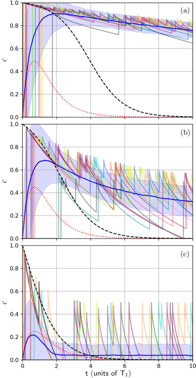
FIG. 6. We plot the evolution of the concurrence C for trajectories arising from inefficient photodetection and including BB-like feedback and measurement reversal as described in the main text; these plots should be compared with Fig. 3, which illustrates the corresponding process under ideal circumstances. We here use symmetric ( \eta_3 = \eta = \eta_4 ) measurement efficiencies \eta = 0.98 (a), \eta = 0.90 (b), and \eta = 0.50 (c). We see that for measurement efficiencies close to the ideal, e.g., as in panels (a) and (b), the average concurrence with feedback always exceeds that without (well approximated by \bar{C}(t) = 2\eta e^{-\gamma t}(1 - e^{-\gamma t}) [24], shown in dotted red). Even in panel (c), where this is no longer true, the ability to maintain any concurrence at long times is still advantageous compared with doing nothing. The upper bound (27) on the concurrence derived in Ref. [24] and shown in dashed black, for the case without feedback, illustrates the extent to which degradation in the measurement efficiency affects the ability to generate entanglement to begin with, and provides another useful reference against which our feedback may be compared.
