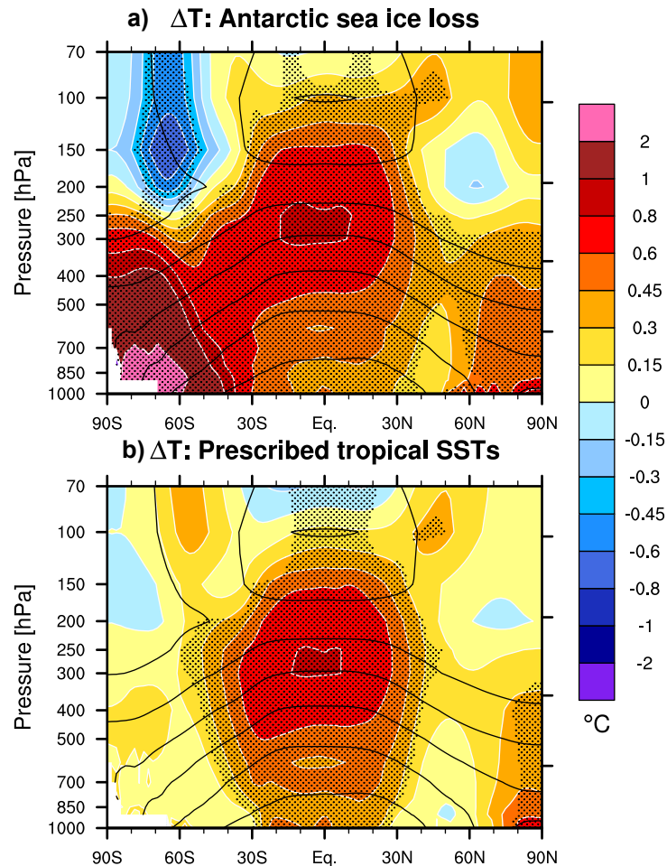
Figure 4. The latitude versus height cross section of the annual mean response of zonally averaged temperature ( ^{\circ}\text{C} ) to (a) Antarctic sea ice loss in the fully-coupled configuration and to (b) prescribed tropical SSTs in an atmosphere-only configuration. Stippling indicates a statistically significant response at 95% confidence.
