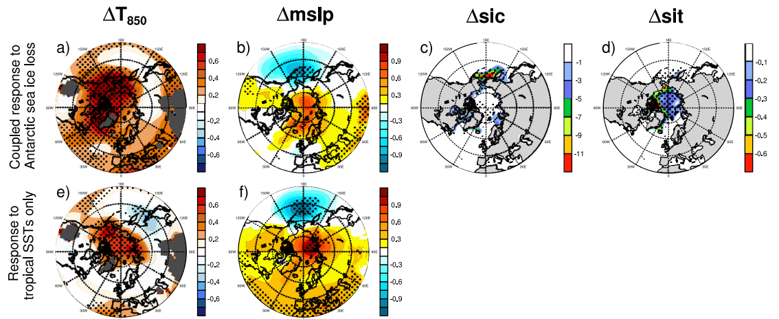
Figure 3. The annual mean response of (a) 850hPa temperature ( ^{\circ}\text{C} ), (b) sea level pressure (hPa), (c) sea ice concentration (in percentage) and (d) sea ice thickness (m) to Antarctic sea ice loss in the fully-coupled simulations. The annual mean response of (e) 850 hPa temperature ( ^{\circ}\text{C} ) and (f) sea level pressure (hPa) to prescribed tropical SSTs (see figure 1) in the atmosphere-only configuration. Stippling indicates a statistically significant response at the 95% confidence level.
