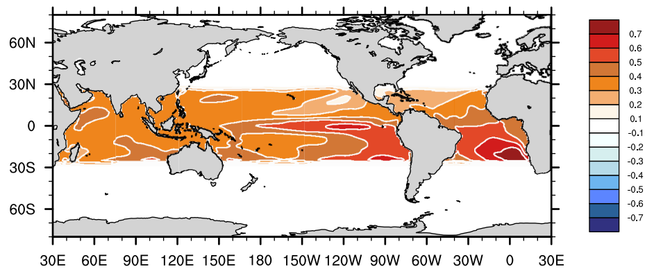
Figure 1. Difference in prescribed SSTs ( ^{\circ}\text{C} ) between the two atmosphere-only runs, from the fully-coupled tropical response to Antarctic sea ice (England et al 2020).
