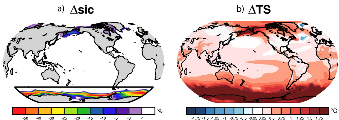
Figure 2. The annual mean response of (a) sea ice (in percentage) and (b) surface temperature (in ^{\circ}\text{C} ) to projected Antarctic sea ice loss. The imposed sea ice loss is shown in the black-bordered box at high Southern latitudes in (a).
