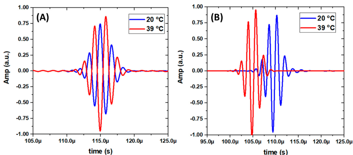
Figure 4. Measured acoustic reflection signals obtained from the setup shown in Figure 3. (A) Reflections. (B) Transmissions. Measured acoustic transmission signals obtained from the setup shown in Figure 3.
