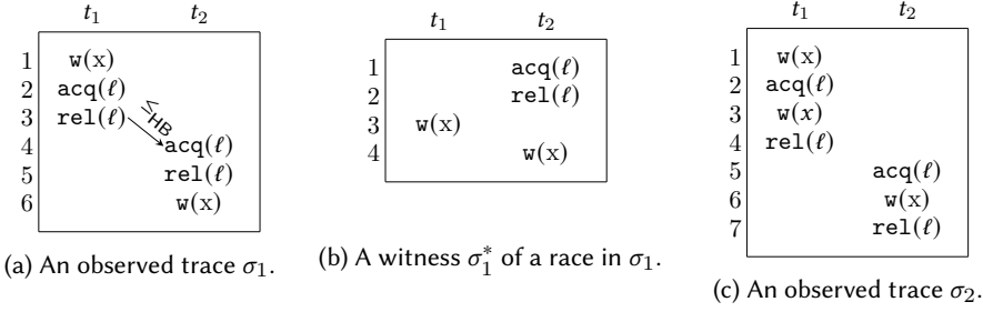
Fig. 1. (1a) shows a trace \sigma_1 with a sync-preserving race ( e_1, e_6 ) missed by \leq_{HB} . (1b) shows a witness that exposes the race. (1c) shows a sync-preserving race ( e_1, e_6 ) that is non-consecutive, due to the intermediate event e_3 .
