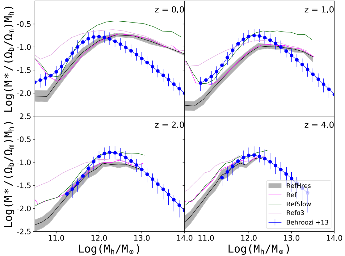
Figure 8. The stellar mass–halo mass functions (SMHMs) at z = 0, 1, 2 , and 4 . We compare the SMHMs from the same set of simulations as in Fig. 3. The solid lines are the running medians of the relation. We also show the scatter of the relation for the RefHres simulation as shaded regions that enclose 68 per cent of all galaxies within each M_h bin. The upturn in the SMHMs below M_h < 10^{11} M_\odot at z = 0 and 1 is a selection effect owing to an artificial stellar mass cut for underresolved galaxies. The blue lines show the empirical best-fitting models from Behroozi et al. (2013) as observational constraints.
