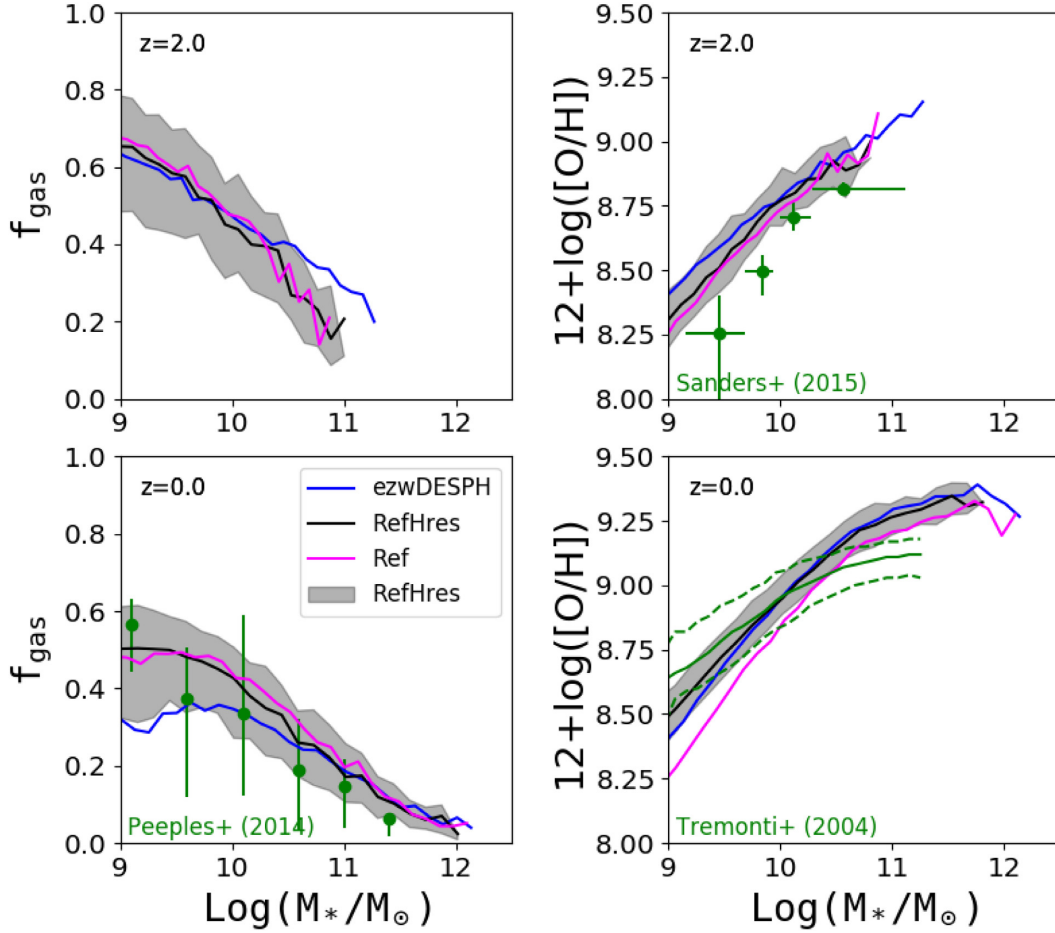
Figure 17. Left-hand panels: cold gas fractions (defined in the text) as a function of stellar mass at z = 2 (upper panel) and z = 0 (lower panel). The observational data in the lower panel are compiled by Peeples et al. (2014), with error bars denoting the 16–84 per cent range. Right-hand panels: gas-phase mass–metallicity relations at z = 2 (upper panel) and z = 0 (lower panel). The z = 2 data are from Sanders et al. (2015) and the z = 0 data are from Tremonti et al. (2004). The shaded area in each panel shows the 16–84 per cent range of the results from the fiducial high-resolution RefHres simulation. We also show the medians from the lower resolution Ref as magenta lines.
