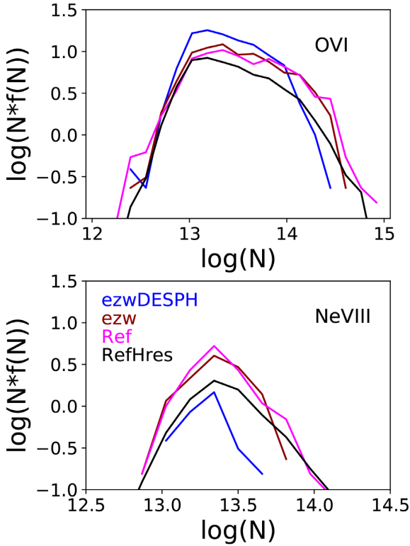
Figure 18. The CDDs of O VI ( upper panel ) and Ne VIII ( lower panel ). We obtain the statistics from random sightlines that span from z = 0.0 to 0.5 as described in the text. Results from the four simulations are colour coded according to Table 1.
