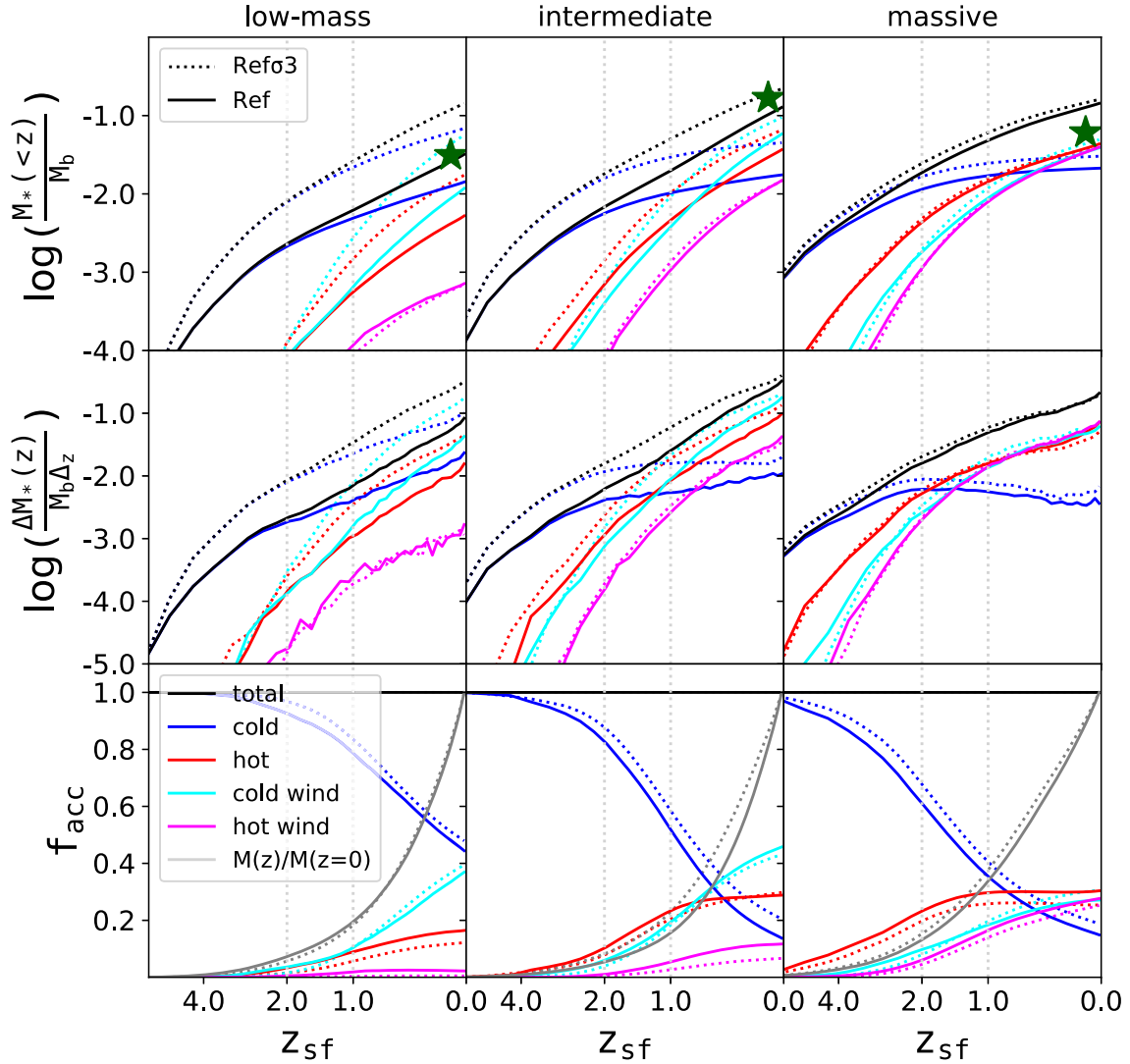
Figure 11. Same as Fig. 10, except that here we compare the Ref and Refσ3 simulations, indicated by the solid and dotted lines, respectively.
