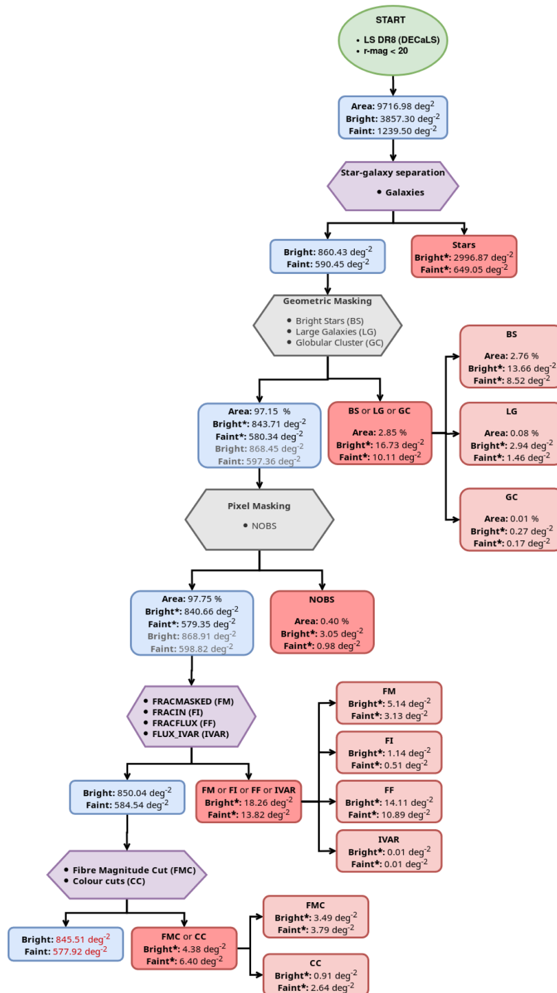
Figure A1. Flowchart showing the spatial and photometric BGS target selections applied to the Legacy Surveys DR8. The spatial selections are shown by grey boxes and are divided into two kinds: one defined by geometric cuts around bright sources, i.e. bright stars (BS), large galaxies (LG), and globular clusters (GC); and the other that is at the pixel level, such as the number of observations (NOBS). The photometric selection of BGS targets is divided into four types and is shown by purple boxes: star–galaxy separation, fibre magnitude cuts (FMCs), colour cuts (CCs), and quality cuts (QCs) that include FRACMASKED, FRACIN, FRACFLUX, and FLUX_IVAR. The blue boxes show the area (in degrees) and the number density (per deg 2 ) of objects retained after each selection, broken down into the numbers for the bright and faint components of the BGS. The red boxes show the equivalent information for the rejected objects. If more than one cut or selection is applied at a given stage, then the darker red boxes show the information about removed objects for the combination of cuts and the lighter red boxes show the corresponding values for each individual cut. The superscript asterisk (*) denotes target densities without correcting for the area removed by cuts up to that point, while densities without a superscript asterisk (*) do take into account the reduction in area.
