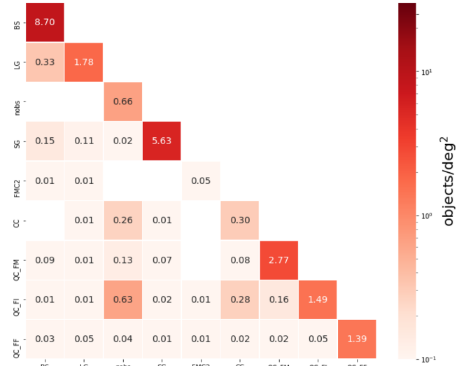
Figure 13. Heat map showing the target density of GAMA galaxies ( z > 0.002 ) that are missed in the BGS. The diagonal shows the number of objects per deg ^2 removed by each of the individual spatial and photometric cuts applied in the BGS, while the off-diagonal entries show the densities of objects removed by both cuts labelled on the x and y axes.
