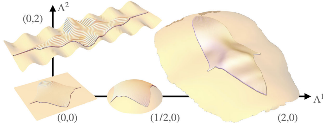
FIG. 3. Inverse design of multiple shapes. A flat uniaxial sheet with two designable system features [ \lambda_i = \exp(c_i \Lambda^i) , i \in \{1, 2\} ] is designed to deform into three target shapes in response to two stimuli \Lambda^1 and \Lambda^2 . The sheet deforms into a sphere and then a facelike mask in response to \Lambda^1 and into a wavy sheet in response to \Lambda^2 . Maximal strains are below 300% and are within experimental reach [45].
