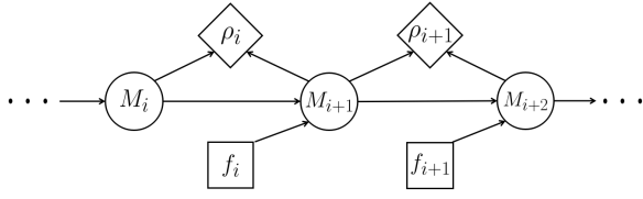
Fig. 2: Illustration of the MDP that underlies PEG. At each time step, the human’s model M_i serves as the state.
