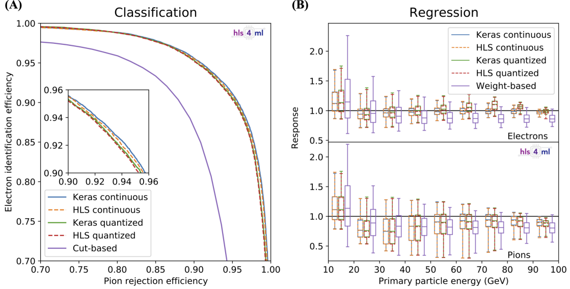
Figure 4: Classification (A) and regression (B) inference performance of the continuous and quantized GARNET-based models and the reference algorithms. Results from the KERAS and HLS implementations are shown for the GARNET-based models. The classification performance is quantified with a ROC curve of electron identification efficiency versus pion rejection efficiency. The inset in (A) shows a close-up view of the efficiency range 0.90–0.96 for both axes. The regression performance is quantified as the response ( E_{\text{pred}}/E_{\text{true}} ) in 10 GeV bins of E_{\text{true}} . The horizontal line in the box corresponds to the median of the distribution, the top and bottom of the box to the upper and lower quartiles, and the upper and lower ends of the whiskers to the 95th and 5th percentiles.
