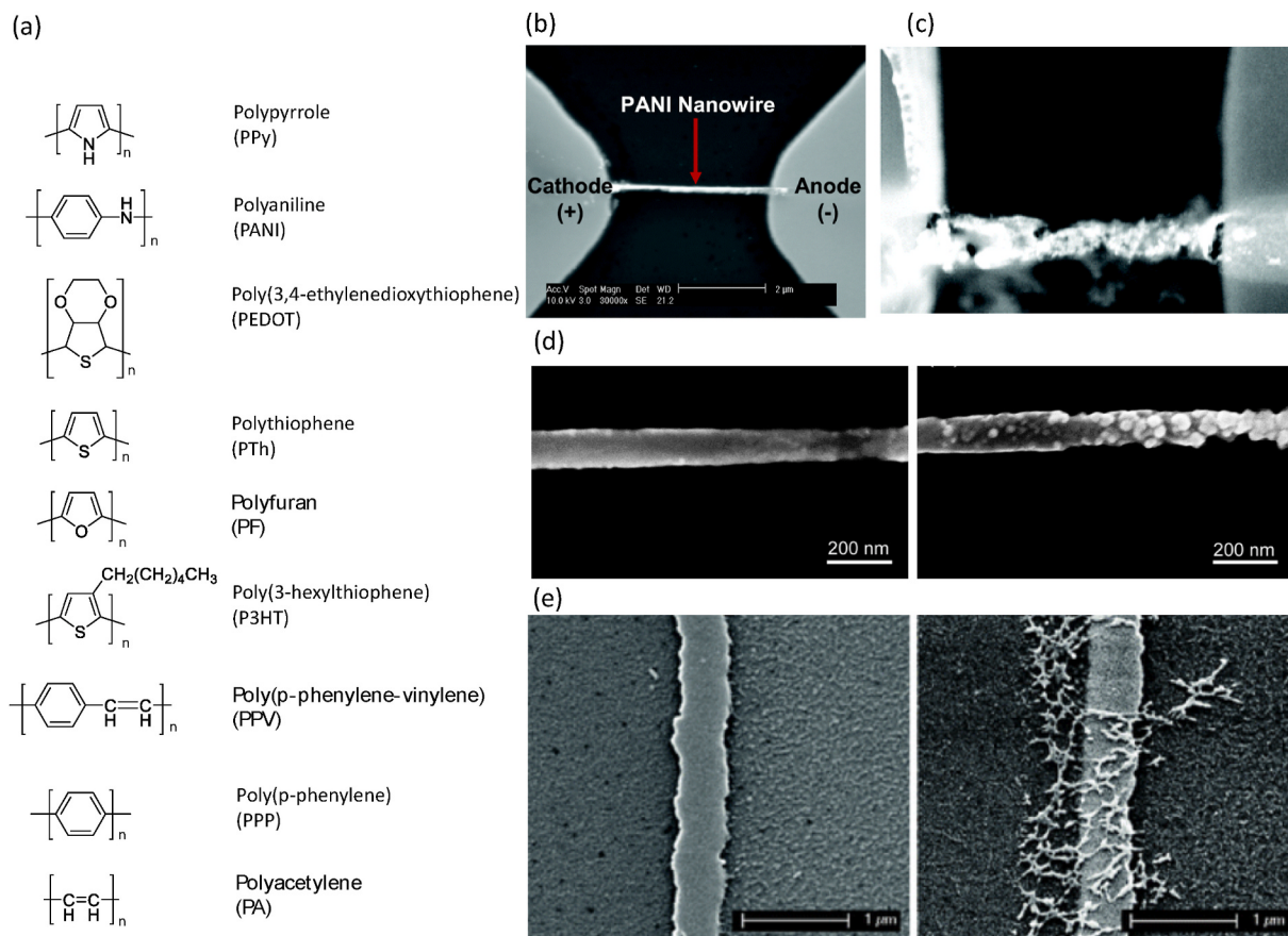
Fig. 4. Molecular structures of common CPNWs and some of their SEM images. (a) Molecular structure of common conducting polymers. (b) SEM image of a 100 nm wide by 4 \mu m long PANI nanowire. Scale bar: 2 \mu m. Reprinted with permission from (Ramanathan et al., 2004). Copyright (2004) American Chemical Society. (c) SEM image of a single avidin-conjugated ZnSe/CdSe quantum dots-embedded PPy nanowire (200 nm wide). Reprinted with permission from (Ramanathan et al., 2005). Copyright (2005) American Chemical Society. (d) SEM images of single PANI NW before (left) and after (right) functionalization with monoclonal antibodies. Adapted from (Lee et al., 2012). (e) SEM images of single PEDOT NWs (left) and net-like structure of virus-PEDOT composite (right). Reprinted with permission from (Arter et al., 2012). Copyright (2012) American Chemical Society.
