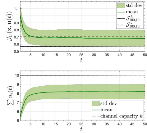
Fig. 5. The top figure shows the empirical performance of our scheme based on average consensus for 100 sample paths J_C(\mathbf{x}, \mathbf{u}(t)) as a function of time t for a system with n = 100 sensors and channel capacity k = 10 . The figure in the bottom shows the corresponding total number of transmitting sensors at a given time t .
