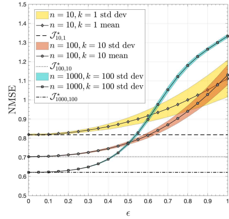
Fig. 4. Monte-Carlo Simulation for the remote estimation system for random perturbations on the mean \mu_i \sim \mathcal{U}[-\epsilon, \epsilon] as a function of \epsilon with n = 10, 100, 1000 sensors and capacity k = 1, 10, 100 .
