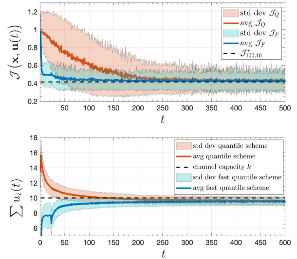
Fig. 7. Performance of the quantile estimation scheme and its accelerated counterpart. The observations are i.i.d. according to a Laplacian distribution, X_i \sim \mathcal{L}(0, 1) , i \in \{1, \dots, n\} . The number of sensors is n = 100 , and capacity is k = 10 .
