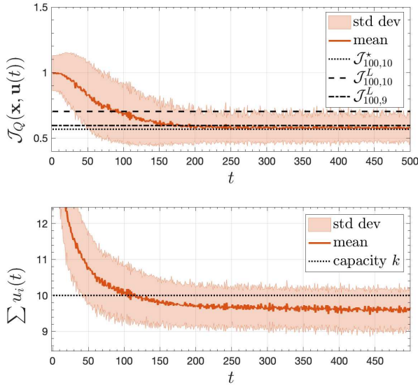
Fig. 6. The top figure shows the empirical performance of our scheme based on quantile estimation for 100 sample paths \mathcal{J}_Q(\mathbf{x}, \mathbf{u}(t)) as a function of time t for a system with n = 100 sensors and channel capacity k = 10 . The figure in the bottom shows the corresponding total number of transmitting sensors at a given time t .
