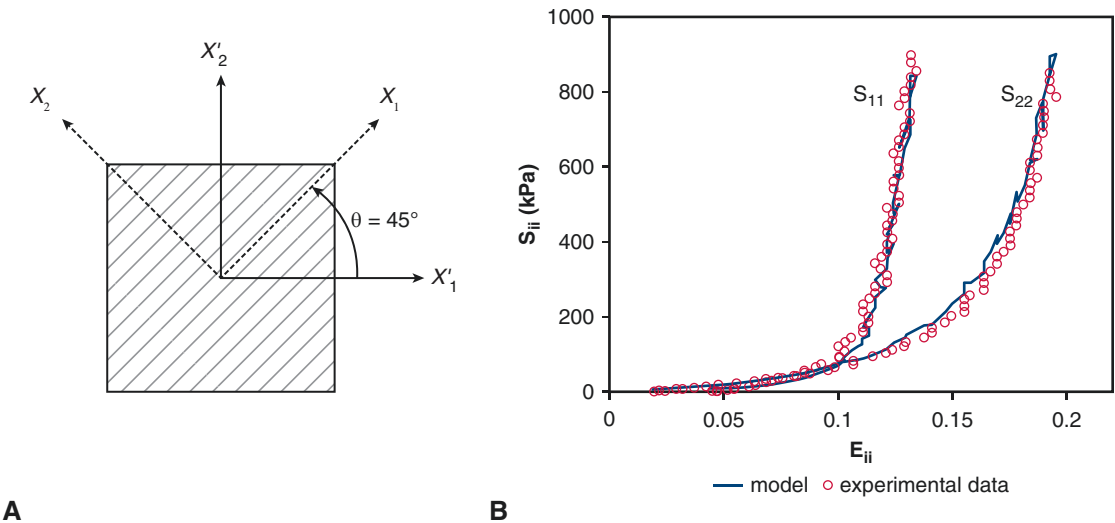
FIGURE E3. Parameter fitting for the valve material models. A, Schematic of the biaxial tensile tests of Kim and colleagues 20 for bovine pericardium tissue specimens to study their material response. X_1 is the preferred mean fiber direction, also shown by gray lines, X_2 is the cross-preferred fiber direction, and X'_1 and X'_2 are the directions in which forces were applied. B, Parameter fitting for the bovine pericardial valve using the equibiaxial data from Kim and colleagues 20 compared with the plot using parameters determined by Kim and colleagues, who used a finite element model of the biaxial test.
