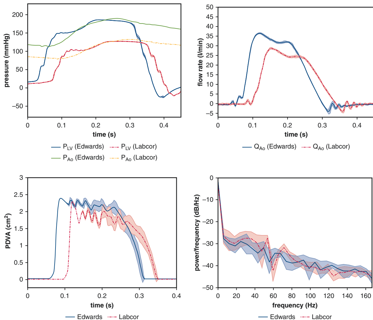
FIGURE E11. Comparison of leaflet kinematics of 25 mm DKA (Labcor Laboratórios Ltd, Belo Horizonte, Brazil) versus Perimount (Edwards Lifesciences, Irvine, Calif) valves. Experimental measurements show variations over 10 consecutive cycles, with shaded regions showing where 95% of the data fall for both valves. We quantify the dominant fluttering frequencies from the experimental projected dynamic valve area (PDVA) signals: 32.74 \pm 3.14 Hz for the Labcor valve and 29.62 \pm 4.7 Hz for the Edwards valve.
