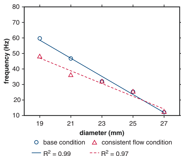
FIGURE 6. Linear regression of fluttering frequency versus valve diameter at physiological Reynolds numbers with consistent operating and flow conditions. Blue circles represent dominant fluttering frequency data with respect to valve diameters obtained for a fixed operating condition but varying flow conditions (quantified by Reynolds number). Red triangles represent dominant fluttering frequency data with respect to valve diameters in which the driving condition is modified to match Reynolds number. Linear regressions show negative relations between frequency response and valve diameter, with proportionality coefficients -5.83 Hz/mm ( blue solid ) and -4.10 Hz/mm ( red dashed ) for consistent operating conditions and flow conditions, respectively.
