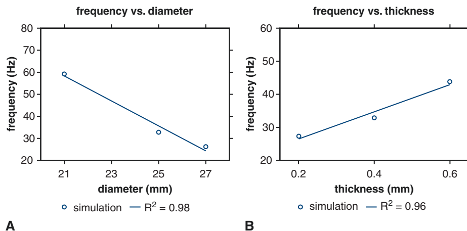
FIGURE 4. Linear regressions of fluttering frequency versus valve diameter and leaflet thickness under consistent operating conditions. Blue circles represent dominant fluttering frequency data from simulations with respect to (A) valve diameter and (B) leaflet thickness under consistent operating conditions. Linear regressions demonstrate that simulations show (A) negative relations between frequency response and valve diameter, with proportionality coefficient -5.65 Hz/mm, and (B) positive relations between frequency response and leaflet thickness, with proportionality coefficient 41.1 Hz/mm.
