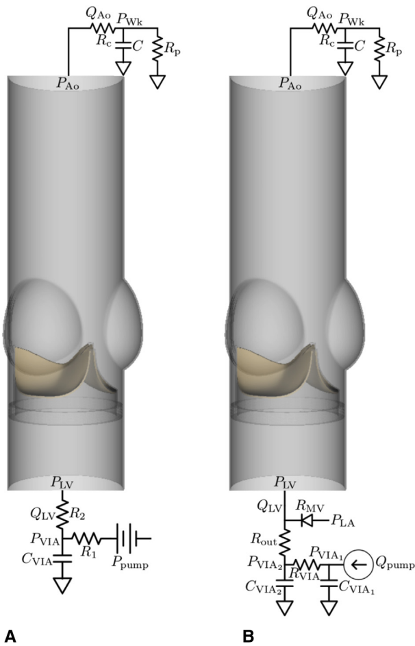
FIGURE E1. Reduced-order models that provide driving and loading conditions. Three-element Windkessel (R-C-R) models are used at the downstream (outlet) for both cases. A, A three-element Windkessel model is used at the upstream (inlet) for simulations that use saline as test fluid. B, A more detailed upstream model is used at the upstream for simulations that use glycerin-based blood analog as test fluid. Because pump flow rate data are available for the experiments that used a glycerin-based blood analog, we are able to modify the pump flow rate to impose consistent flow conditions necessary for the study reported in Figure 7.
