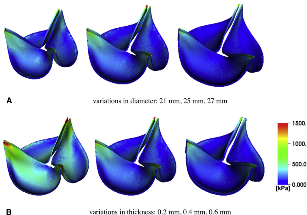
FIGURE E10. Stress analyses for 25 mm valves with different leaflet thicknesses. A, Comparison of von Mises stress between valves with a fixed thickness (0.4 mm) and different diameters (21 mm, 25 mm, 27 mm). B, Comparison of von Mises stress between valves with a fixed diameter (25 mm) and different thicknesses (0.2 mm, 0.4 mm, 0.6 mm). The results in panel A indicate that for a fixed thickness, the larger valve experiences smaller stress on the leaflets during diastole. This suggests that larger diameter valves may have an advantage in durability both during systole and diastole. The results in panel B indicate that for a fixed diameter, the thinner valve leaflets experience higher stress loads.
