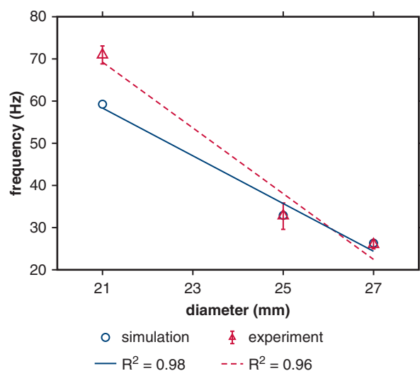
FIGURE 3. Comparison of linear regressions of fluttering frequency versus valve diameter between simulations and experiments. Blue circles represent dominant fluttering frequency data from simulations that match the different experimental operating conditions of each device. Red triangles represent dominant fluttering frequency data with respect to valve diameters obtained from experimental projected dynamic valve area measurements. Linear regressions demonstrate that both simulation and experiment show negative relations between frequency response and valve diameter, with proportionality coefficients -5.65 Hz/mm and -7.79 Hz/mm, respectively, for simulation ( blue solid ) and experiment ( red dashed ).
