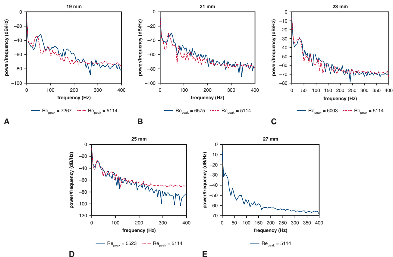
FIGURE E9. Analysis of simulated leaflet kinematics for valves with different diameters at physiological Reynolds numbers with consistent operating and flow conditions. A through E, frequency analyses of leaflet fluttering obtained using a glycerin-based blood analog. Blue solid lines represent the simulation results obtained for a fixed operating condition but varying flow conditions (quantified by Reynolds number [ Re_{peak} ]). Red dashed lines represent results in which the driving condition is modified to match Re_{peak} . The dominant fluttering frequencies for different Reynolds number cases are: A, 59.70 and 47.86 Hz; B, 46.75 and 35.82 Hz; C, 32.00 and 31.75 Hz; D, 25.32 and 25.24 Hz; and E, 12.12 Hz. Smaller-diameter valves show higher frequency leaflet fluttering.
