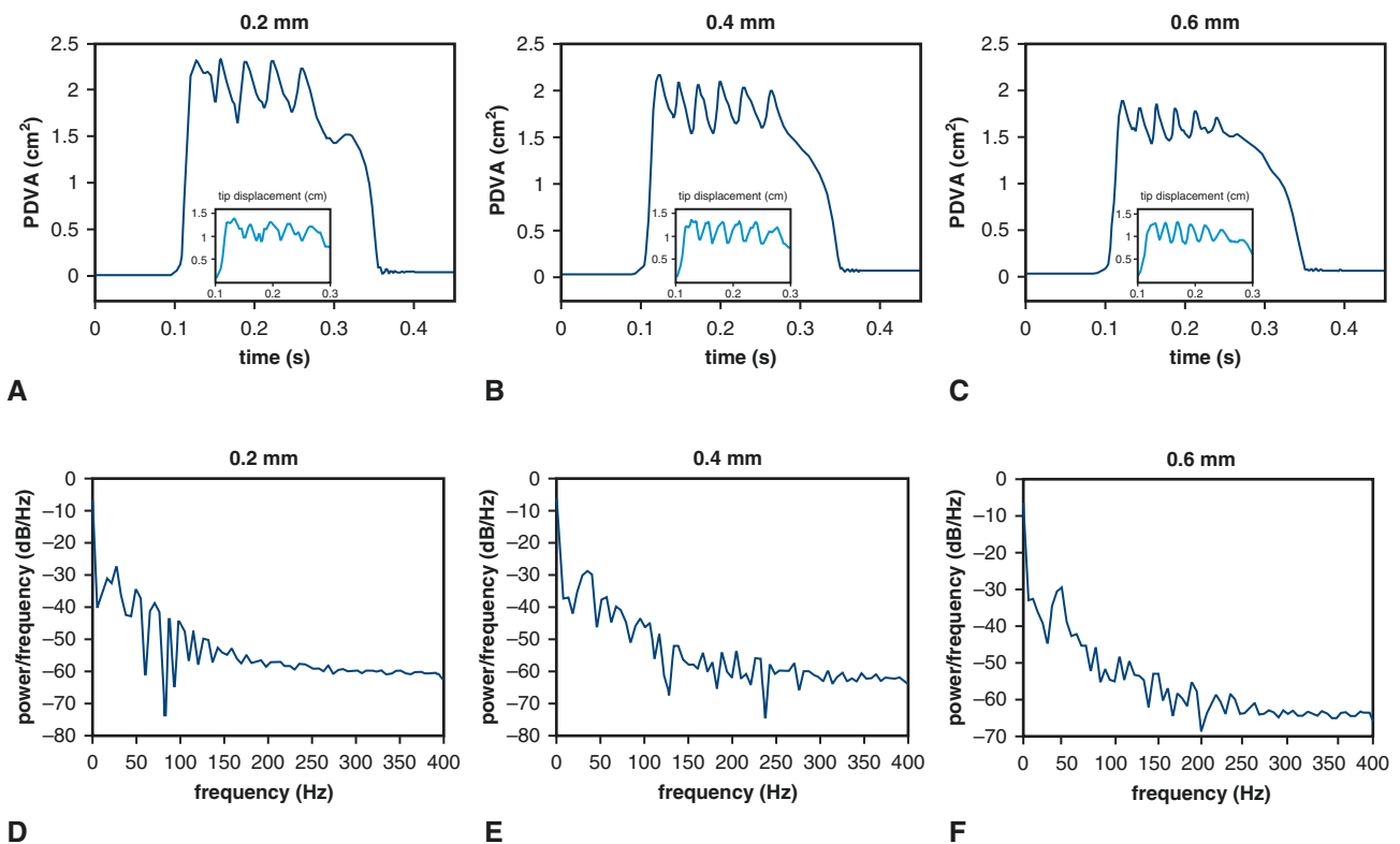
FIGURE E8. Analysis of simulated leaflet kinematics for valves with different leaflet thicknesses under consistent operating condition. A through C, Projected dynamic valve area (PDVA) and tip displacements are obtained from the computational models using the operating condition for the 25 mm valve but with varying leaflet thicknesses. D through F, Frequency analyses quantify the dominant fluttering frequencies: D, 27.40 Hz (0.2 mm); E, 32.88 Hz (0.4 mm); and F, 43.84 Hz (0.6 mm). These results suggest that at a fixed diameter, valves with thinner leaflets flutter at lower frequencies.
