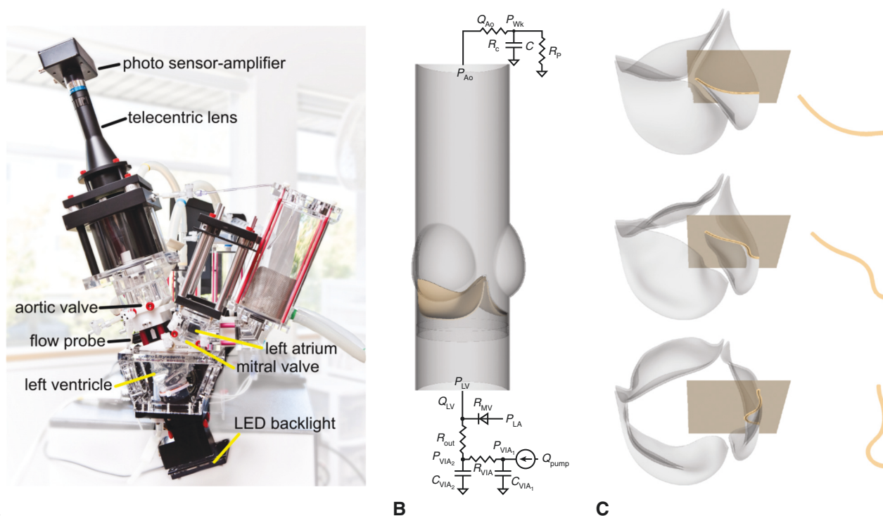
FIGURE 1. Experimental and computational pulse duplicators. A, Customized pulse duplicator with electro-optical subsystem for measuring aortic valve projected dynamic valve area. B, Computer model of the aortic valve test section in the pulse duplicator with pericardial bioprosthetic heart valve (BHV) and reduced-order models of the upstream and downstream system components. C, Three-dimensional rendering of the model BHV leaflets. Leaflet kinematics are detailed on the highlighted cross-sections in Figures E5 and E6 .
