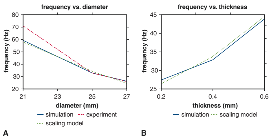
FIGURE 5. Comparison of leaflet fluttering frequency versus scaling model for different bioprosthetic heart valve (BHV) diameters and leaflet thicknesses. Panel A compares fluttering frequencies obtained for different BHV diameters to frequencies determined from the scaling law. Panel B compares fluttering frequencies obtained for different BHV leaflet thicknesses to frequencies determined from the scaling law. The results are consistent in both cases.
