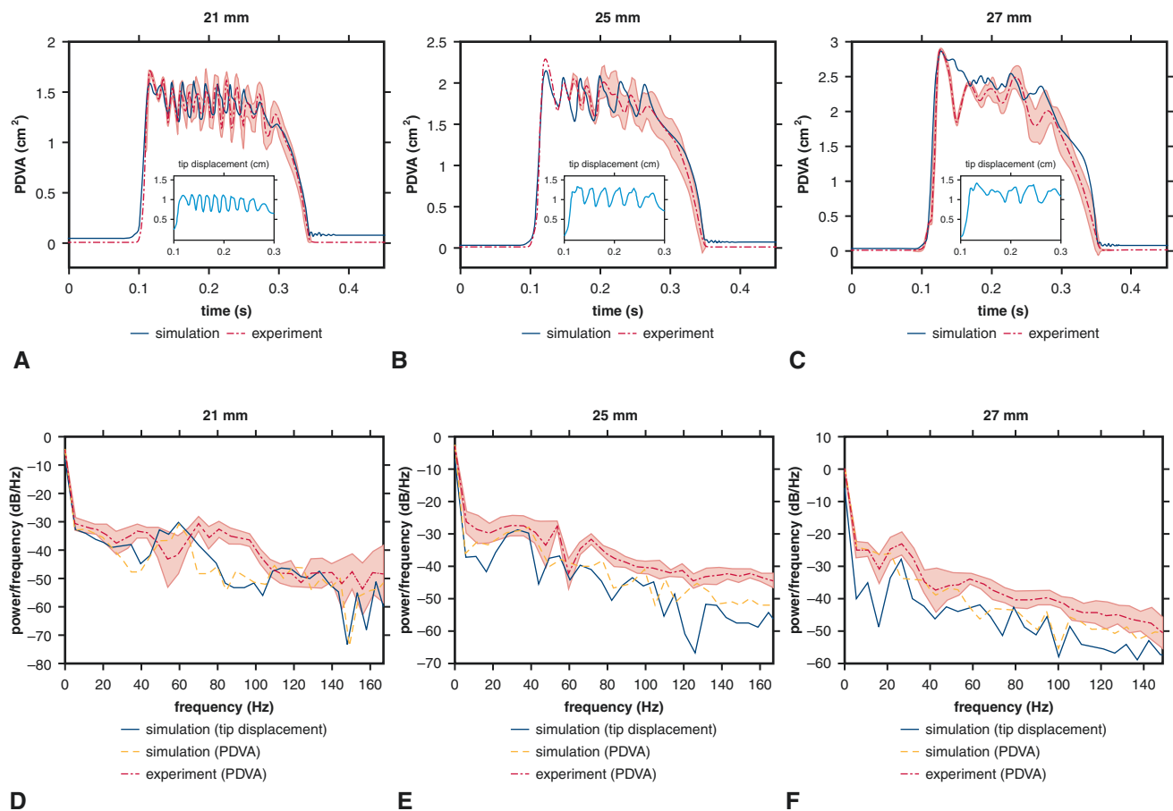
FIGURE 2. Analysis of experimental and computational leaflet kinematics. Experimental measurements show variations over 10 consecutive cycles, with shaded regions showing where 95% of the data fall. For each available valve diameter, the computer model matches the experimental operating conditions, which are different for each valve. Panels A through C compare simulated results to the experimental data for projected dynamic valve area (PDVA), and insets show the simulated displacement of the leaflet tip from the center of the valve. Panels D through F show frequency analyses. Dominant fluttering frequencies from experimental and simulated PDVA signals and simulated tip displacement signals are, respectively, D, 70.97 \pm 2.11 Hz, 59.63 Hz, 59.26 Hz; E, 32.74 \pm 3.14 Hz, 38.62 Hz, 32.88 Hz; and F, 26.03 \pm 1.04 Hz, 21.05 Hz, 26.32 Hz. Smaller valves clearly show markedly higher fluttering frequencies.
