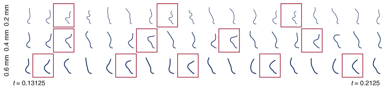
FIGURE E6. Detailed leaflet kinematics obtained from the computational model with different leaflet thicknesses. Time series of leaflet cross sections (see Figure 1, C) for different valve thicknesses for a fixed valve diameter (25 mm) described in Figure 6. Red boxes indicate the times when the peak tip displacement of the leaflet occurs. The valve with the thickest leaflets (0.6 mm) shows more frequent leaflet bending than the thinnest leaflets (0.2 mm).
