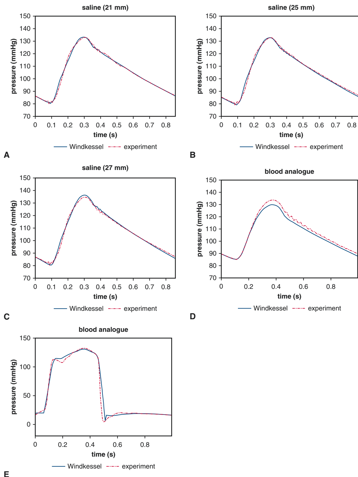
FIGURE E2. Reduced-order model fits of the experimental pressure data for the saline and glycerin-based analog cases. Panels A through D show the fits of the experimental downstream pressure data for both saline and glycerin-based blood analog cases. These fits are obtained using the nonlinear optimization routine fmincon in MATLAB by comparing experimental values of downstream pressure to the computed downstream pressure from the reduced-order model with experimental values of downstream flow rate as inputs to the model. Panel E shows the experimental upstream pressure data for glycerin-based blood analog case. The fit is obtained by comparing experimental values of upstream pressure to the computed upstream pressure from the reduced-order model with experimental values of left atrial pressure and pump flow rate as inputs to the model.
