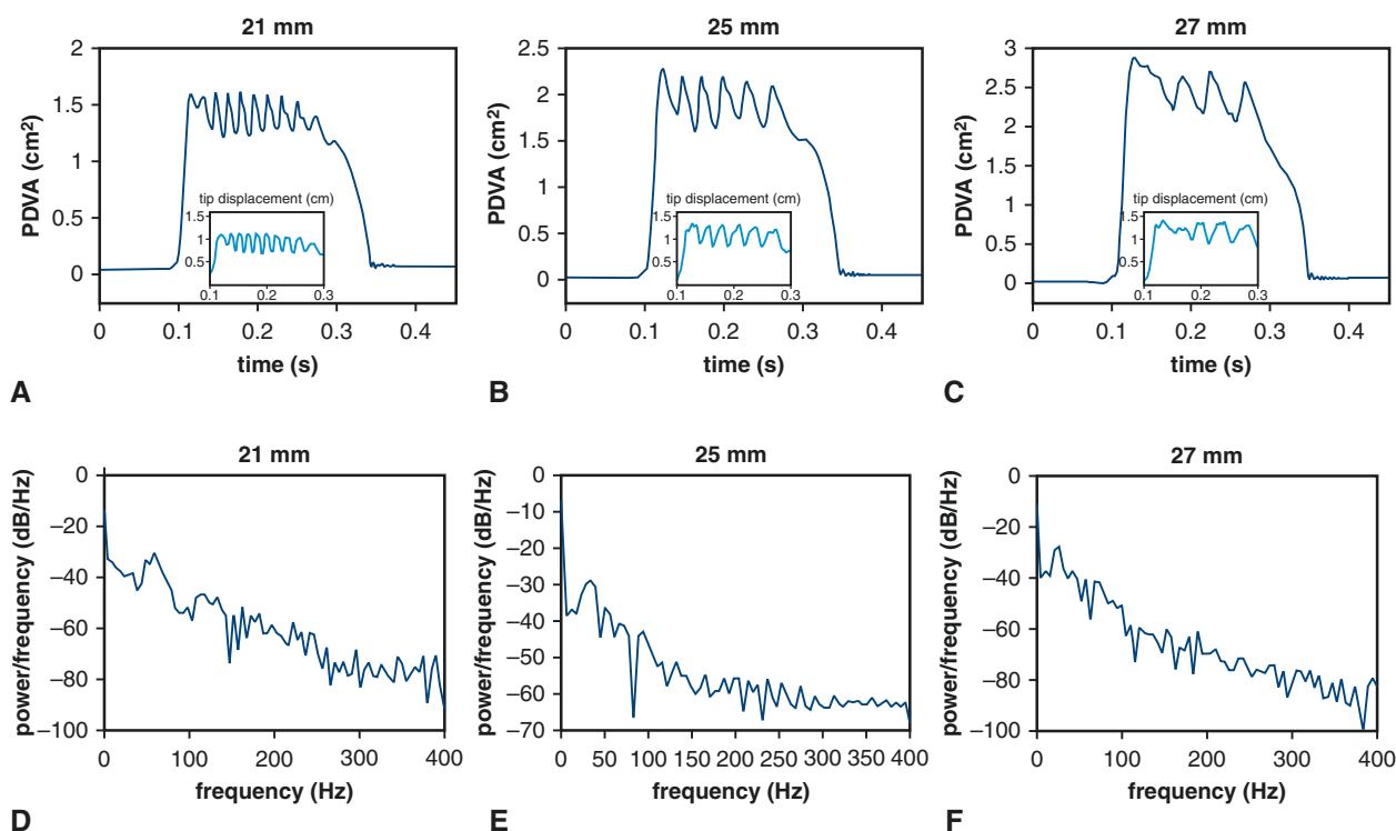
FIGURE E7. Analysis of simulated leaflet kinematics for valves with different diameters under consistent operating conditions. A through C, projected dynamic valve area (PDVA) and tip displacements are obtained from the computational models for each valve diameter using volumetric flow rates and pressure loads corresponding to the 21 mm valve in Figure 2, A . D through F, Frequency analyses quantify dominant fluttering frequencies: D, 59.26 Hz; E, 32.88 Hz; and F, 26.32 Hz. These frequencies are identical to those reported in Figure 2 .
