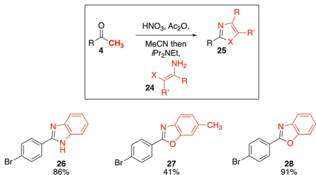
Fig. 3 One-pot conversion of an aromatic methyl ketone to heterocycles. Yield based on heteroatom nucleophile.
