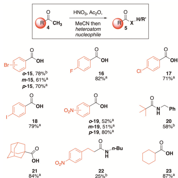
Fig. 2 One-pot acetyl nitrate-mediated conversion of methyl ketones to carboxylic acid derivatives. Examples varying the methyl ketone substrate. a Yield based on methyl ketone. b Yield based on heteroatom nucleophile.
