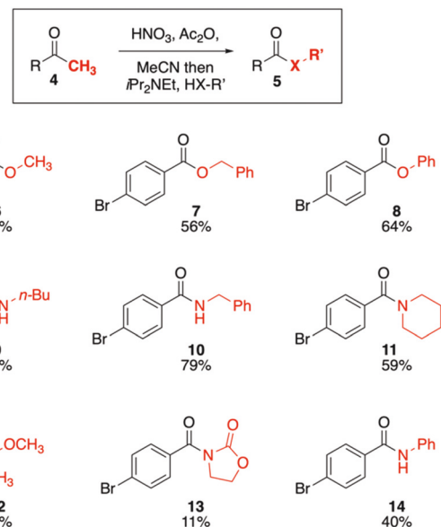
Fig. 1 One-pot acetyl nitrate-mediated conversion of methyl ketones to carboxylic acid derivatives. Examples varying the heteroatom nucleophile. Yield based on heteroatom nucleophile.
