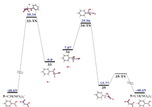
Fig. 5 Differences in total free energy between various states as compared to 33 + OH - . Includes solvent and ZPE corrections. The product from both pathways is benzoic acid.
