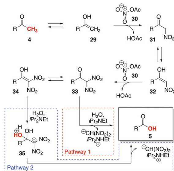
Fig. 4 Proposed mechanism for acetyl nitrate-mediated synthesis of carboxylic acid derivatives from methyl ketones.
