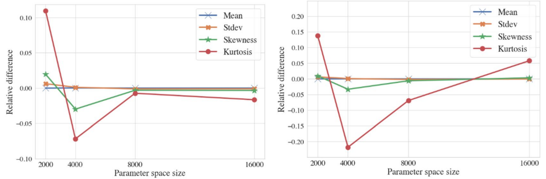
(a) Statistical convergence check for the depplaning time
