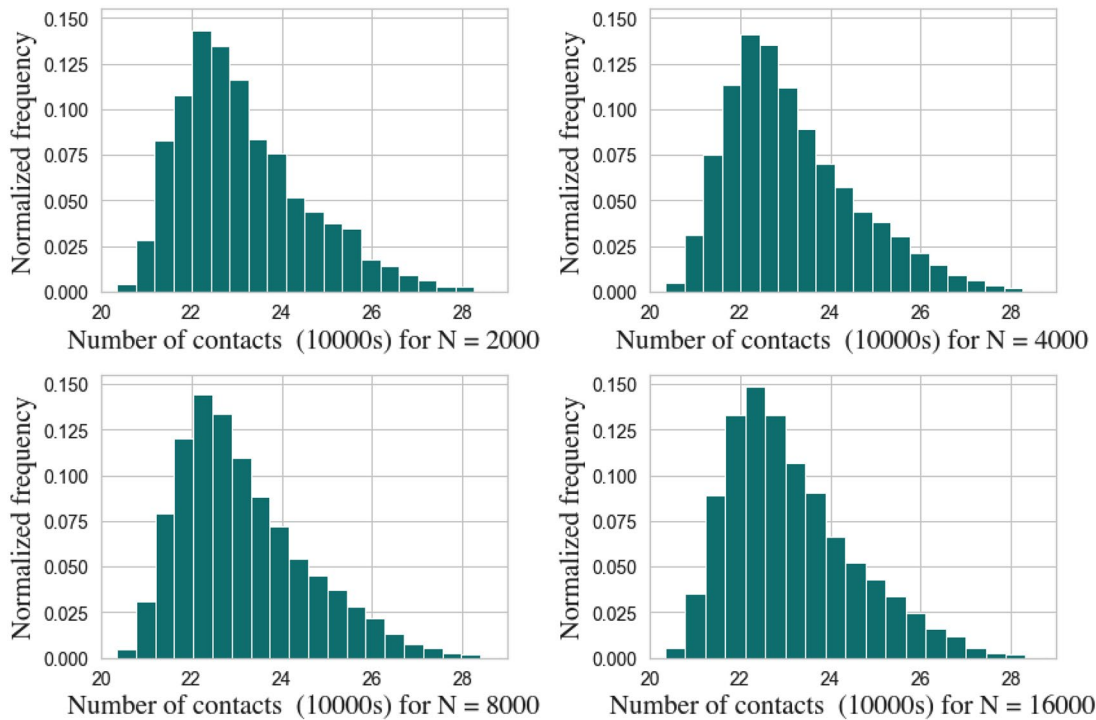
Figure 2: Histograms of the number of contacts.
