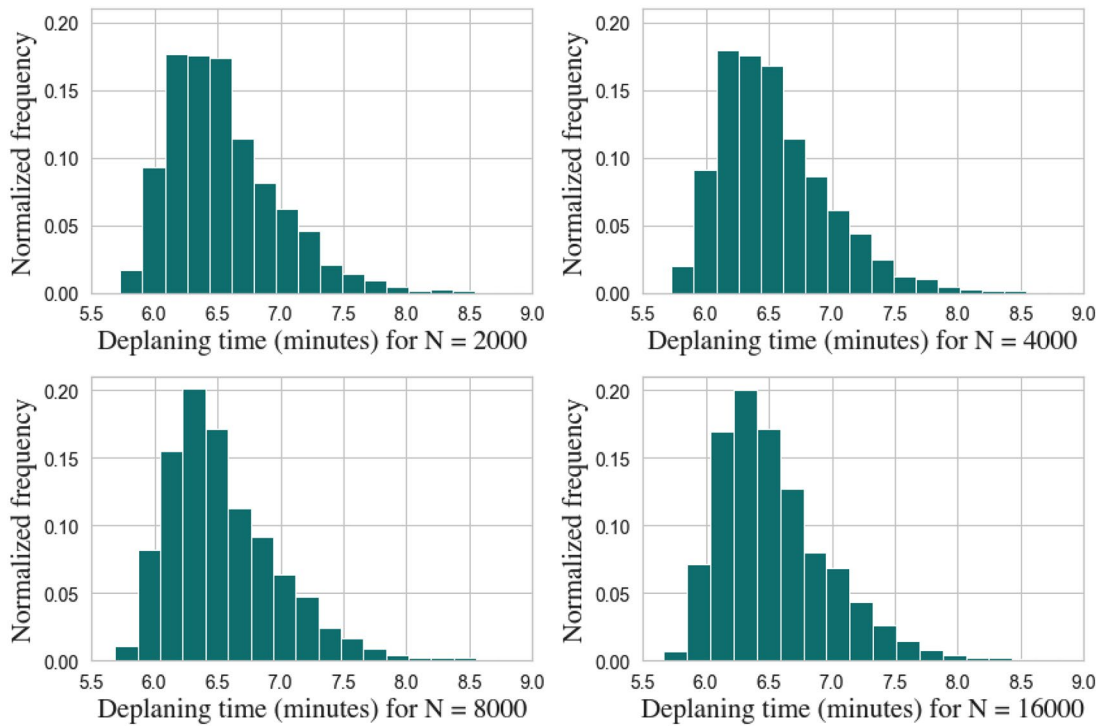
Figure 1: Histograms of deplaning times.
