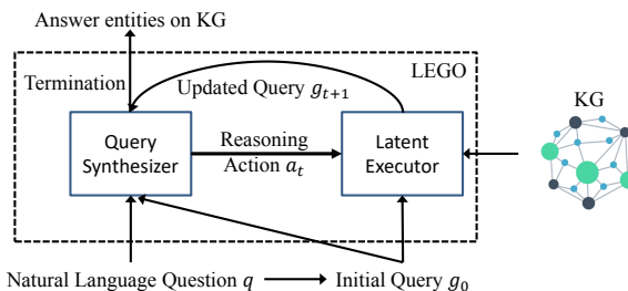
Figure 1. LEGO answers a question by iteratively performing execution-guided query synthesis and latent query execution.
