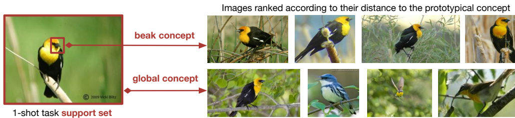
Figure 4: Top row shows images with beak concept embeddings most similar to the prototypical beak. Bottom row shows images ranked according the global concept that captures whole image. COMET correctly reflects local similarity in the underlying concept of interest, while global concept often reflects environmental similarity.
