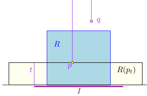
Fig. A.4: The point p is in R , but q is not.
