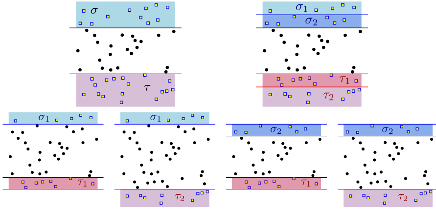
Fig. 2.2: Illustration of the proof of Theorem 1.
