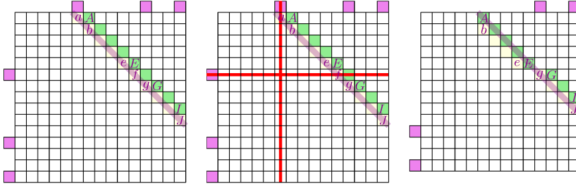
Fig. 2.1: Illustration for the proof of Lemma 1.
