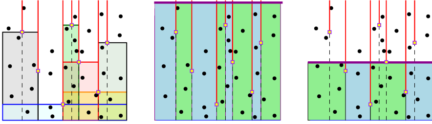
Fig. 2.5: Merging intervals during the sweeping.
