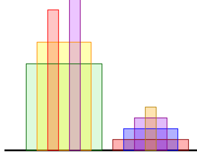
Fig. 2.4: A laminar family of rectangles
