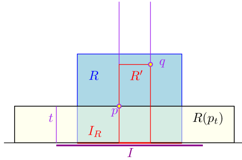
Fig. A.3: The points p and q are both in R .
