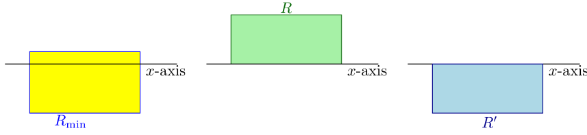
Fig. 2.3: A rectangle, its folding, and its reflection.
