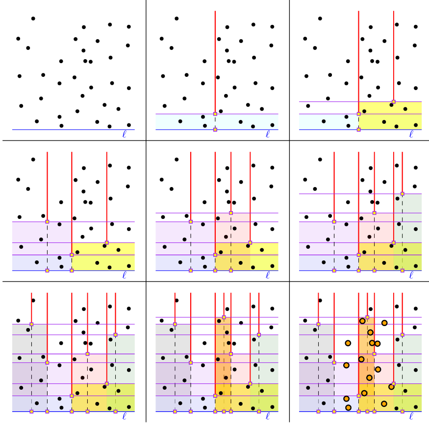
Fig. A.1: An illustration of Lemma 2. The last pane on the right shows the point set associated with the last interval being split.
