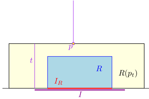
Fig. A.2: p is not in R .
