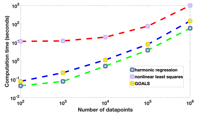
Fig. 6. Log-log comparison of computation time for harmonic regression (green), GOALS (blue), and nonlinear least squares (red) as a function of the size N of the synthetic dataset (the noisy data with gaps from Figs. 2 – 4). GOALS is comparable in expense to harmonic regression but significantly less expensive than nonlinear least squares, with a more pronounced difference for small N . The asymptotic slopes give estimates of the complexity ( \sim N^{1.1209} , \sim N^{1.2672} , \sim N^{1.1877} , respectively). Algorithms were implemented in MATLAB on a 2016 Macbook Pro (2.9 GHz Intel Core i7).
