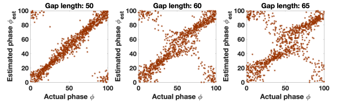
Fig. 5. GOALS phase estimates for the synthetic dataset when the gap is lengthened (up to 50, 60, 65 of 100 data consecutively removed, resp.). Noise bias \alpha is fixed at 0.75. Phase estimates become noisier as the gap becomes larger, becoming heavily biased when roughly two-thirds of data are discarded.
