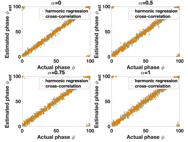
Fig. 1. Phase estimates \phi_{est} compared to true phase \phi for harmonic regression and cross-correlation on a synthetic dataset with missing data. For each of 1000 trials, a uniformly random phase \phi was used to generate data d_i from a 100-period sinusoidal signal f(t, \phi) and i.i.d. noise \beta_i sampled from a Gaussian with mean \alpha and variance 1; one third of the data were then removed uniformly at random, with harmonic regression and cross-correlation used to estimate phase from the remaining data. Results are shown for four values of the noise bias \alpha . Regardless of \alpha , both methods recover phase to good accuracy (i.e., along the diagonal \phi_{est} = \phi ).
