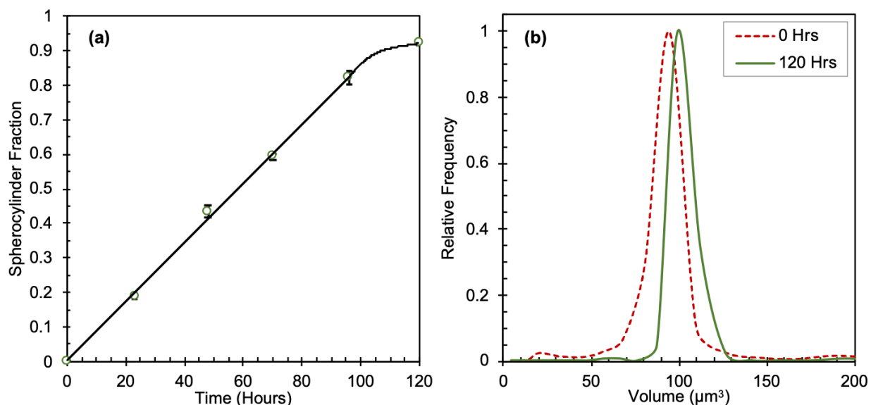
Figure 5. Quantitative analysis from SEM images of the ratio of spherocylinder to spherical morphology versus stirring time at room temperature (a) and volume distribution comparison for the 120-hour sample of spherocylinders versus the original dispersion of spheres (b)
