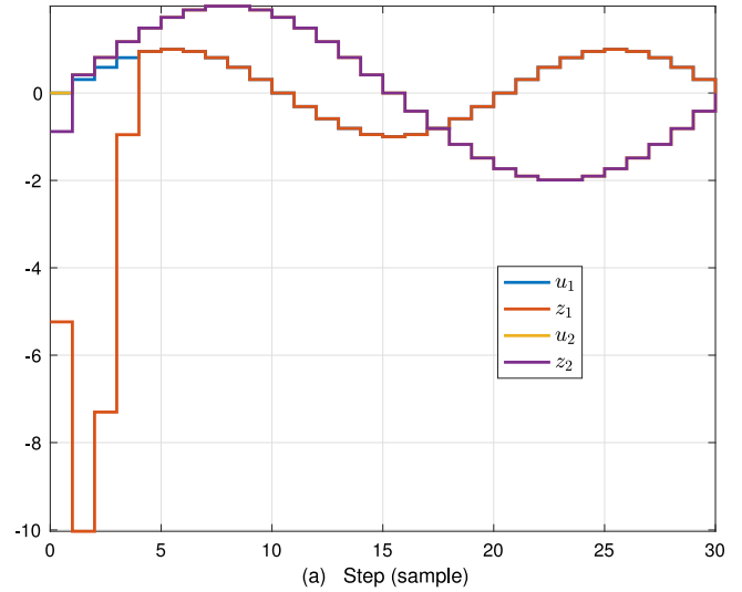
Fig. 3. Input and output of (6), (7), where u = [u_1 \ u_2]^T and z = [z_1 \ z_2]^T . Note that, for all k \geq 4 , z_1(k) = u_1(k) , and, for all k \geq 1 , z_2(k) = u_2(k) . Hence, for all k \geq 4 , z(k) = u(k) .
