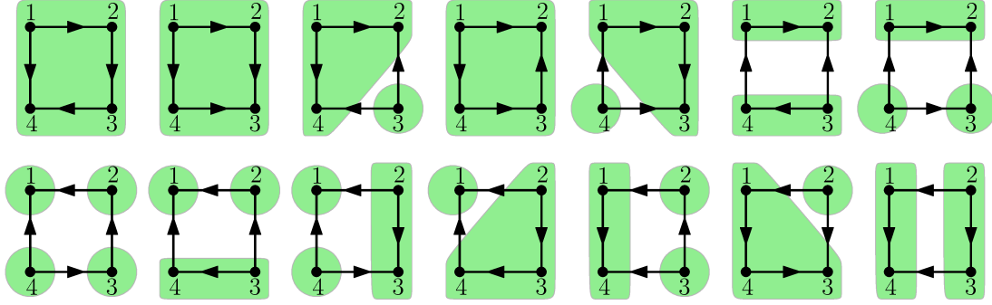
FIGURE 2. The source-components of the 14 acyclic orientations of the graph of Figure 1.
