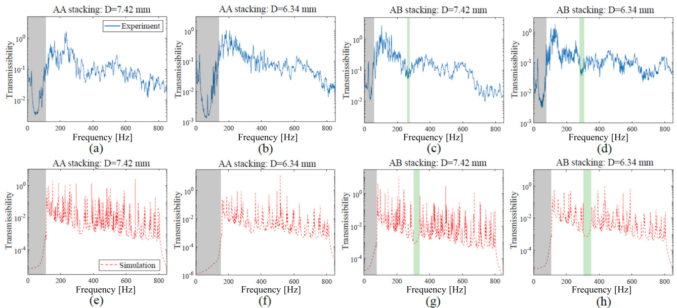
FIG. 5. Experimental results. (a)–(d) Transmissibility vs frequency plots obtained from vibrometry data for (a),(b) AA stacking and (c),(d) AB stacking, for different interlayer distances. The plots reveal a foundation band gap, whose width depends on the interlayer distance and can be tuned by twist. For sufficiently strong interlayer interactions, a second band gap associated with symmetry breaking is switched on by twisting the layers from AA to AB stacking. (e)–(h) Transmissibility plots obtained from full-scale simulations for the same stacking conditions and interlayer distances, correlating well with the experimental results.
