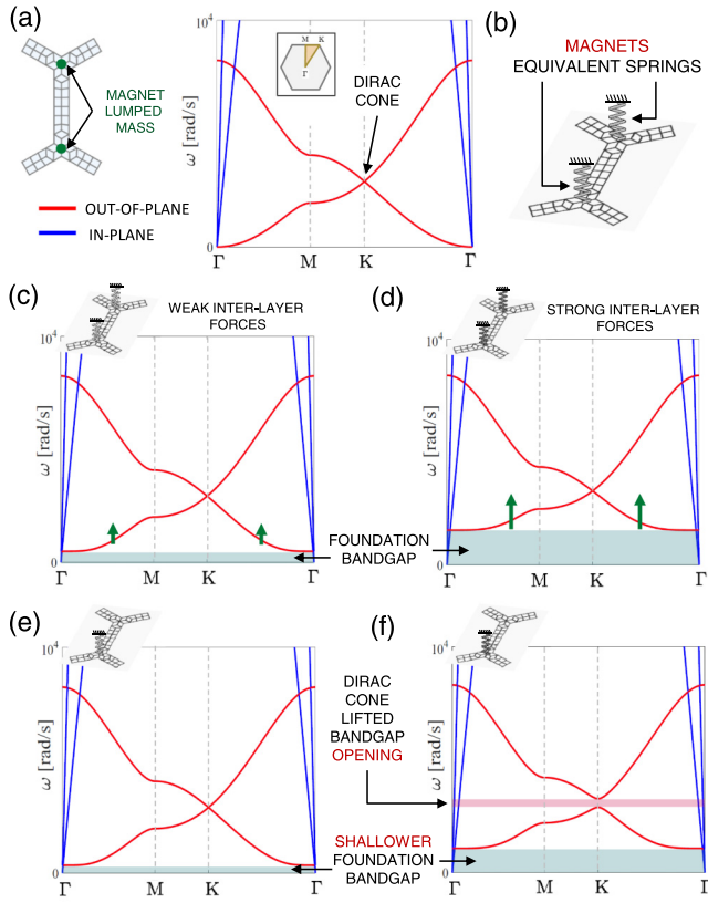
FIG. 3. (a) Evolution of band diagram upon changes in twist angle and interlayer distance. (a) Baseline case of single layer: FEM model of unit cell; band diagram with in-plane (blue) and out-of-plane (red) modes, featuring Dirac cone at K point of the Brillouin zone. (b) Unit cell with elastic foundation (AA stacking case shown). (c) AA stacking with large interlayer distance (weak magnetic forces), with up-shifting of the flexural mode and opening of a foundation band gap. (d) AA stacking with smaller interlayer distance (stronger magnetic forces), resulting in increase of the foundation band-gap width. (e) AB stacking with weak magnetic forces, resulting in reduction of the foundation band-gap width. (f) AB stacking with strong magnetic forces, resulting in increase in foundation band-gap width and opening of finite-frequency band gap due to space inversion symmetry (SIS) breaking.
