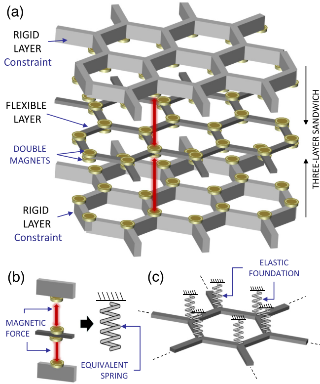
FIG. 1. Magnetomechanical multilayer analog of graphene bi-layer. (a) Three-layer sandwich stacking. (b) Equivalent spring model for the magnetic interactions. (c) Inner layer modeled as a single layer on an elastic foundation.
