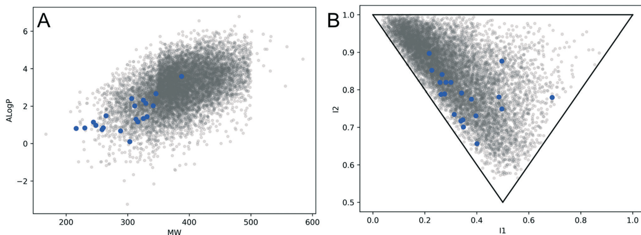
Fig. 3 Comparison of molecular properties for this compound collection (blue) and a commercially available epigenetic compound collection (grey). A: Molecular weight vs. \text{ALogP} . B: Principal moment of inertia plot. The commercially available epigenetic library is shown in grey and our focused library described is shown in blue. \text{ALogP} and principal moment of inertia (PMI) were calculated in RDKit. PMI represents the three-dimensional shape of a molecule where rod-like molecules are in the top left, disc-like molecules are at the lower middle, and sphere-like molecules are in the top right of the plot.
