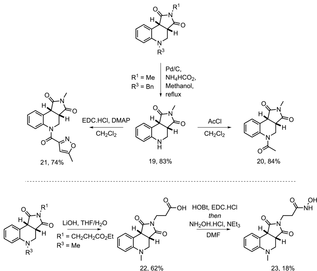
Scheme 2 Derivatizations of the tetrahydroquinoline scaffold.
