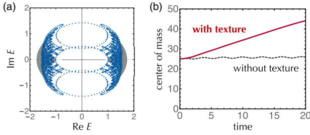
FIG. 1. Non-Hermitian topological phenomena in two dimensions. The periodic boundary conditions are imposed along both directions ( L_x = 50 , L_y = 20 ; \gamma = 0.5 ). (a) Complex spectra in the presence ( \Theta = 1 , blue dots) and absence ( \Theta = 0 , gray regions) of the spatial texture. (b) Time evolution of the wave packet center of mass along the x direction. The initial state is prepared to be |\psi(0)\rangle \propto \sum_y |x = L_x/2, y\rangle .
