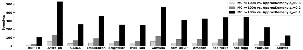
Figure 3: Speed-up by our MC algorithm over ApproxKemeny.
