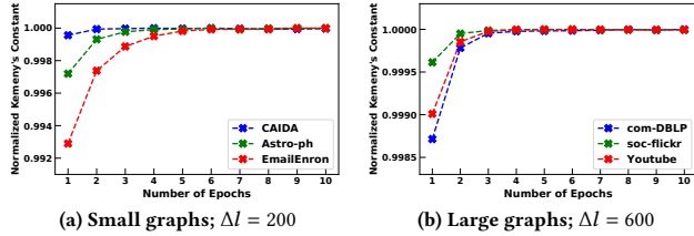
Figure 5: (Normalized) Kemeny's constant estimated by our MC algorithm with varying chain length l .
