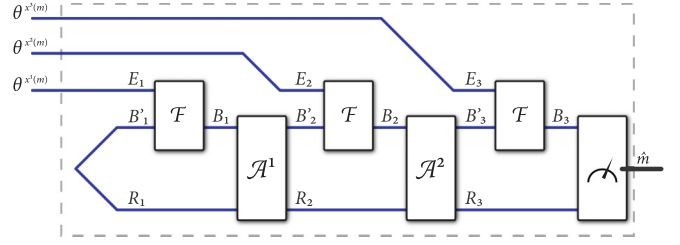
FIG. 2. The figure depicts how a quantum rebound protocol for an environment-parametrized collection with associated environment states \{\theta_E^x\}_{x \in \mathcal{X}} can be rewritten as a protocol that tries to decode the message m from the environment states \theta_{E^n}^{x^n(m)} . All of the operations inside the dashed lines can be understood as a measurement on the states \theta_{E^n}^{x^n(m)} .
