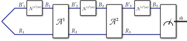
FIG. 1. The DW model of quantum reading from Ref. [28]. Beyond the physical setup of quantum reading, this can also be understood in the most abstract sense as a quantum rebound protocol, in which a call to the channel collection or “channel box” \{\mathcal{N}_{B' \rightarrow B}^x\}_{x \in \mathcal{X}} is made three times and the most general quantum strategy for decoding the message m is employed.
