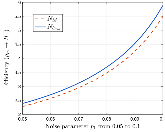
FIG. 1. Comparison between N_{\theta_{\max}}(\rho_{\text{in}} \rightarrow H_+) and N_M(\rho_{\text{in}} \rightarrow H_+) for input \rho_{\text{in}} = (1 - p_1 - p_2)|H_+\rangle\langle H_+| + p_1|H_-\rangle\langle H_-| + p_2|H_i\rangle\langle H_i| with p_2 = 1/10 .
