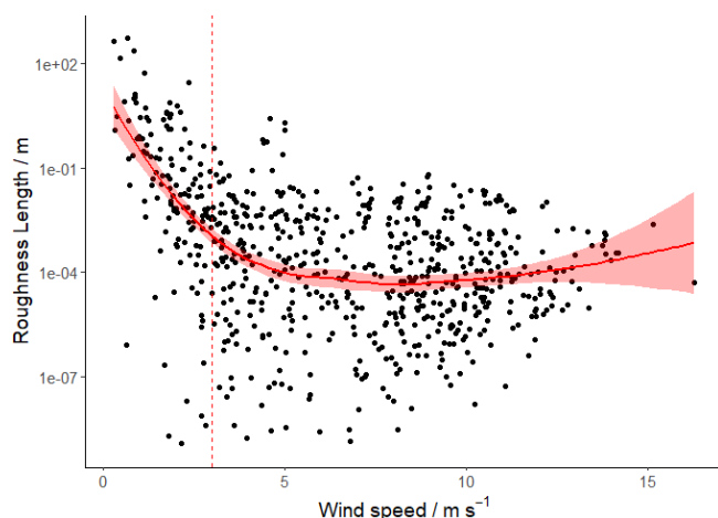
Figure 5. Roughness length for each averaging interval (black dots) with a smoothed local regression (LOESS) line (solid red, 95 % confidence interval shaded). Points left of the 3 \text{ m s}^{-1} filter threshold (dashed red) are not used in subsequent discussions of oceanic deposition velocity. The y axis is limited for clarity, with 17 points < 10^{-9} \text{ m} not shown.
