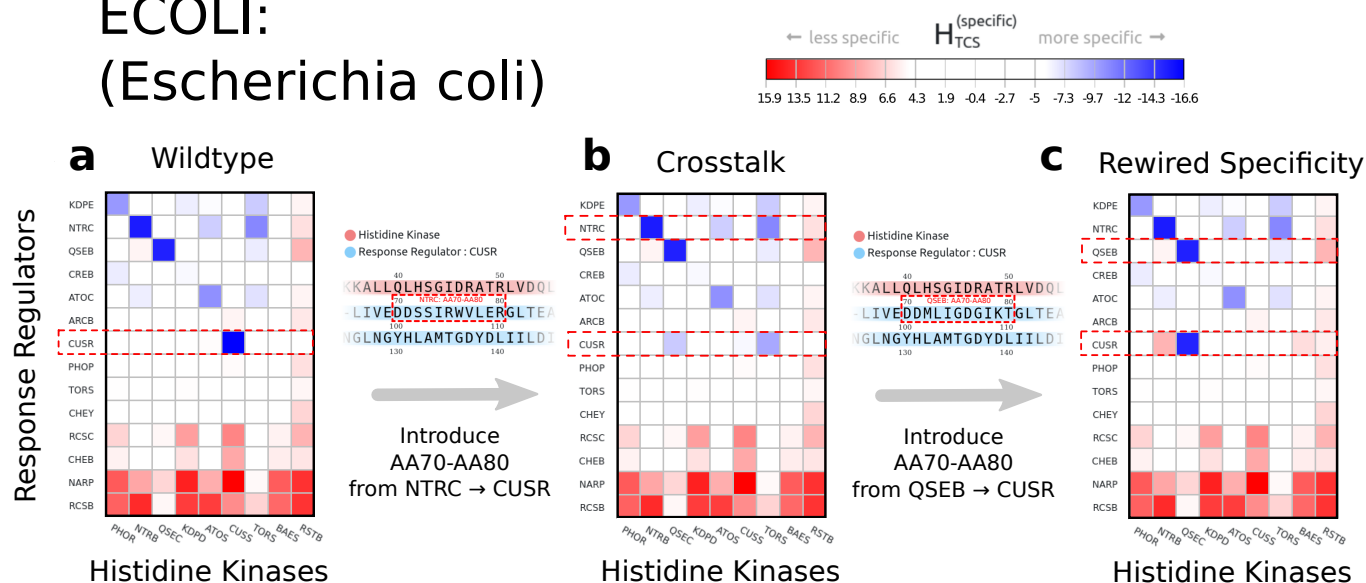
Figure 4. (a) One of the many use cases for the web server is the exploration and in silico change of specificity. In this example, we identify the response regulator cusR as the interaction partner of the histidine kinase cusS indicated by the lowest value in our Hamiltonian. (b) The transfer of a significant sequence portion of the response regulator ntrC does not disrupt the initial interaction and introduces cross-talk through a second interaction partner. (c) Alternatively, the introduction of a sequence portion of the response regulator qseB into cusR disrupts the initial interaction and rewires the interaction towards qseC .
