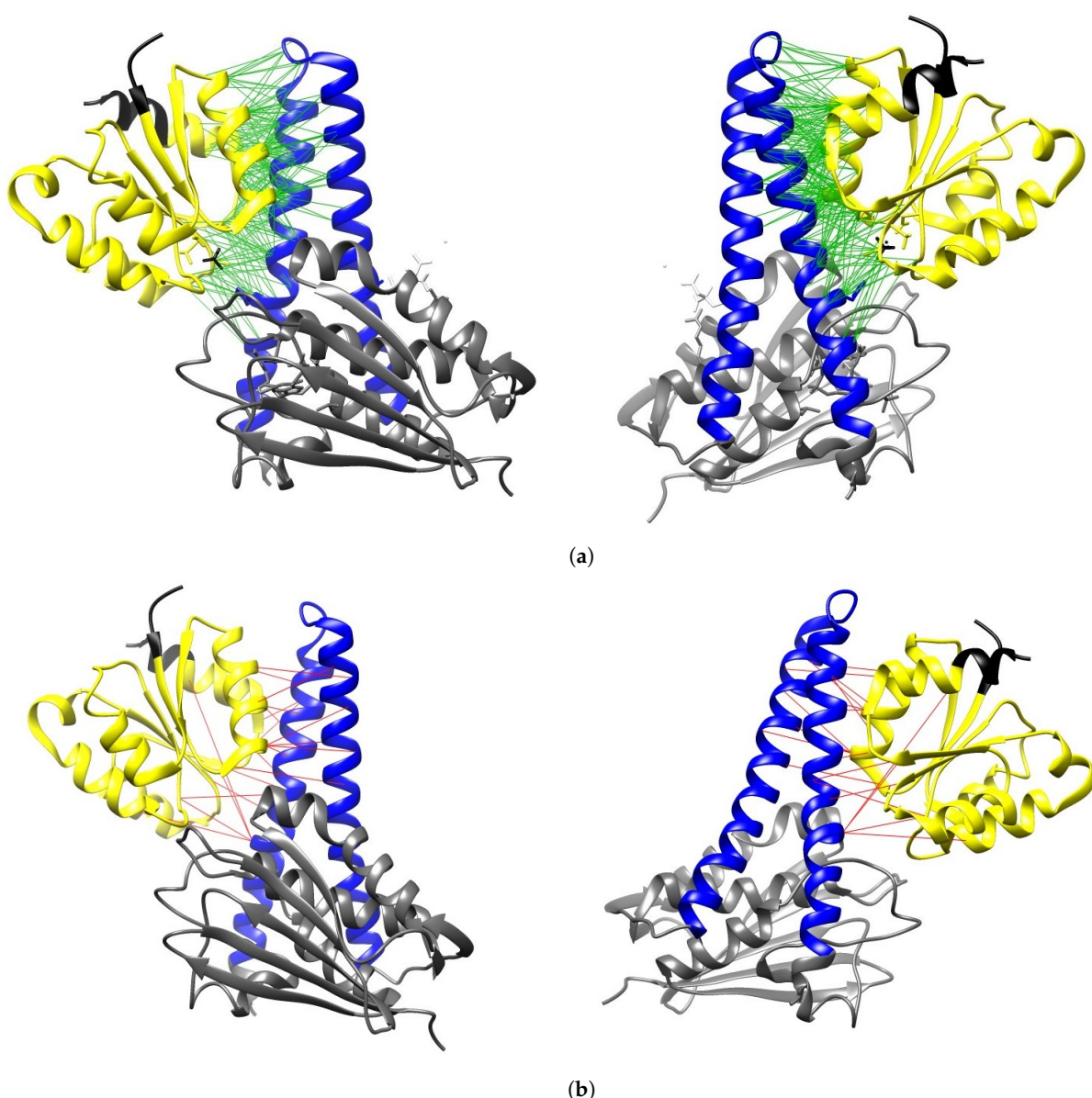
Figure A4. Gray structures show the HK residues lying outside of the HisKA domain. Black structures show the RR residues lying outside the REC domain. The blue structure represents the HisKA domain, and the yellow structure represents the REC domain. Green pseudobonds show contacts within 12 Angstroms C_{\alpha} to C_{\alpha} . Red pseudobonds show the top 20 DCA couplings. The distribution of DCA couplings indicates that the model does not show biases towards subregions of the interface. (a) All contacts within 12 Angstroms as found in the structure viewed from two different positions, left and right faces; (b) Top 20 interfacial DI contacts as viewed from left and right faces.
