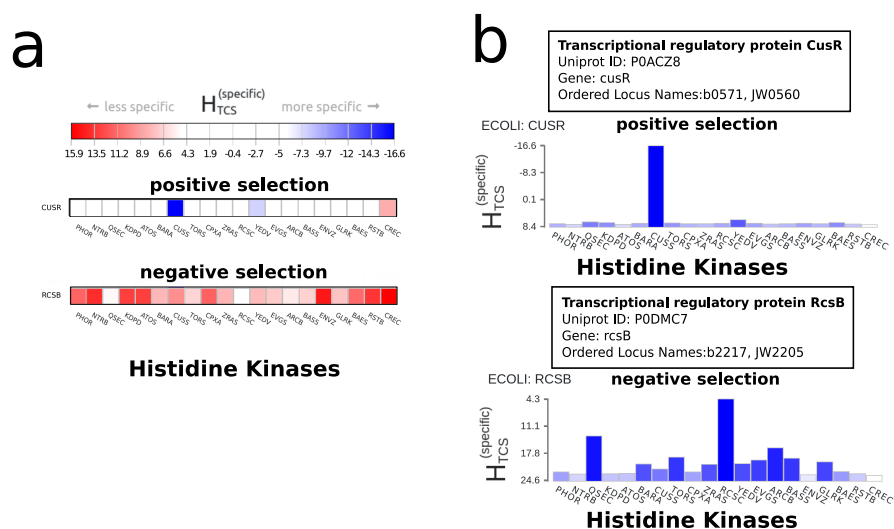
Figure 5. Negative selection in Escherichia coli strain K12 (ECOLI). (a) Heatmap view for the response regulators cusR and rcsB . In cusR , a single interaction between cusR and the histidine kinase cusS is dominant. This is a case of positive selection between two interacting partners. In rcsB , the majority of interactions are reported as having a low specificity. Even though the interaction between rcsB and the histidine kinase rcsC is not reported as having a high specificity, it will be the dominant interaction for rcsB as there is no stronger interaction partner for signal transduction. This is an example of negative selection. (b) Histogram view for the response regulators cusR and rcsB . From these histograms, it becomes clear that cusR - cusS (top) and rcsB - rscC (bottom) are the dominant interactions.
