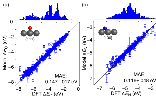
Fig. 5 TinNet models for other adsorbates/facets. DFT-calculated vs. TinNet-predicted (a) ^*\text{O} adsorption energies at the atop site of {111}-terminated alloy surfaces and (b) ^*\text{N} adsorption energies at the hollow site of {100}-terminated alloy surfaces for all 10-fold test sets, along with a histogram of data sampling. Note: the color scheme of atoms includes red (O), blue (N), and dark gray (metal). The error bar corresponds to the standard deviation of the error estimates from 10 final models.
