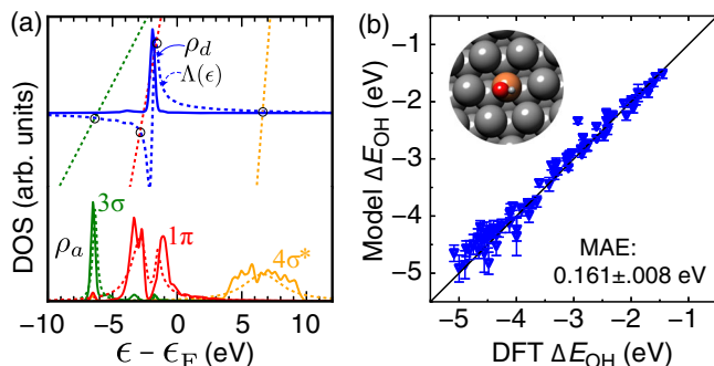
Fig. 3 Out-of-sample validation of the TinNet model. a Projected density of states \rho_d onto the OH 3 \sigma , 1 \pi , and 4 \sigma^* orbitals from DFT calculations (solid) and TinNet models (dashed), taking Cu 1 /Ag(111) as an example (Ag: dark gray, Cu: brown). The graphical solution to the Newns–Anderson model is also shown, in which the intersections of the adsorbate line y = (\epsilon - \epsilon_a)/\pi\beta V_{ad}^2 for each orbital with the Hilbert transform \Lambda(\epsilon) of the density of d -states \rho_d represent the adsorbate-substrate bonding and antibonding states (2 localized roots) for 1 \pi and the resonance state (1 localized root) for 3 \sigma and 4 \sigma^* . b DFT-calculated vs. TinNet-predicted *OH adsorption energies for out-of-sample single-atom alloys. A broad range of transition-metal atoms (26 in total) were used as the single-site substitute of the coinage metal host, i.e., Cu, Ag, and Au. The error bar corresponds to the standard deviation of the error estimates from 10 final models.
