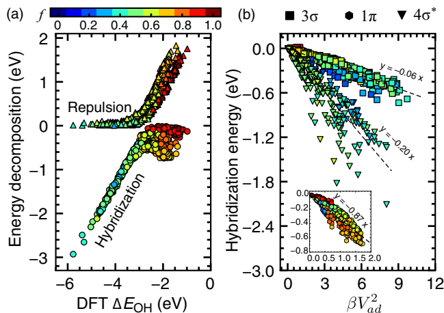
Fig. 4 Physical insights into chemical bonding. a Orbital hybridization and Pauli repulsion contributions from the metal d -states to the ^*\text{OH} adsorption energies on all 10-fold test sets deconvoluted by the TinNet models. b The TinNet-predicted coupling integral squared \beta V_{ad}^2 for 3\sigma , 1\pi , and 4\sigma^* orbitals linearly correlate with the corresponding orbital hybridization energy ( R^2 : 0.93, 0.87, and 0.89, respectively). Regression lines with the intercept at 0 are shown. To avoid overlap, the 1\pi data are plotted in the inset. All markers are color-coded according to the theoretical d -band filling f of the ^*\text{OH} adsorption site.
