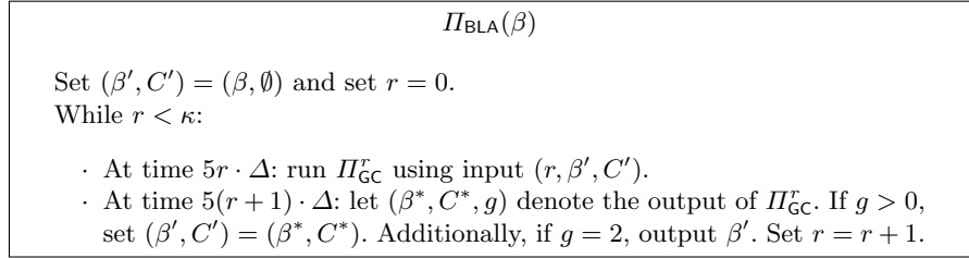
Fig. 9. A block-agreement protocol \Pi_{BLA} with security parameter \kappa , from the perspective of party P_i .
