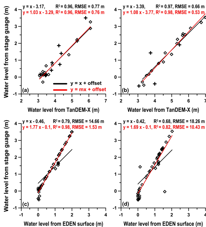
Fig. 3. Calibration plots of the absolute water level maps in (a) August 26, 2015 and (b) August 31, 2015. Assuming that there is a single offset between two observations ( y = x + \text{offset} ), the estimated offsets between InSAR and stage station observations were used to adjust the derived water level instead of reference points. The black solid-line plots show excellent agreement (degree of determination > 0.95 ), and the estimated RMSE is 0.77 and 0.66 m, respectively. The symbol “+” marks outliers omitted from the calibration offset calculations because of mostly low coherence. The red line’s best-fit plots show a very similar linear pattern with a single offset fit model. A best-fit in black solid-line and a single offset fit in red is displayed to compare hourly water level stage station measurements with interpolated EDEN surface map using daily stage station data in (c) August 26, 2015 and (d) August 31, 2015. Although both measurements show a good correlation (degree of determination of 0.68–0.79), systematic gradients ( \sim 1.7 ) causing worse RMSE level ranges from 14.66 to 18.26 m have been estimated. Thus a single offset fit model shows a divergent pattern to a best-fit model.
