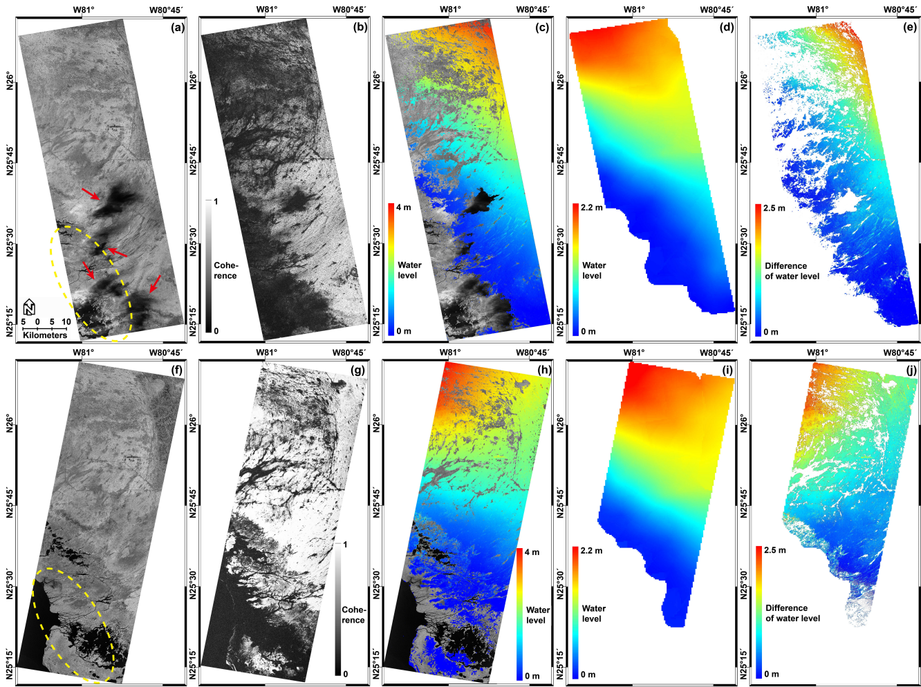
Fig. 2. (a) and (f) Backscattered amplitude images and (b) and (g) coherence maps of the August 26 (top) and 31 (bottom) 2015 acquisitions. Severe coherence degradations were detected in the high and dense vegetated areas and tree islands [yellow dot ellipse in (a) and (f)]. Significant radar signal attenuation by atmosphere was identified in the middle and lower part of images, marked by red arrows in (a), leading to a loss of coherence. (c) and (h) Extracted absolute water level maps scaled from 0 to 4 m. (d) and (i) EDEN interpolated water surface maps obtained from the daily median stage data [14]. (e) and (j) Residual map between the InSAR-derived and EDEN water surfaces showing deviation up to about 2.5 m. Linear ramps in both residual maps indicate systematic disagreements between the two maps.
