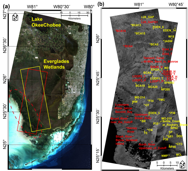
Fig. 1. (a) Landsat-8 operational land imager (OLI) optical image of southern Florida showing the TanDEM-X SAR tracks collected on August 26 (yellow rectangle) and 31 (red rectangle), 2015. Red ellipse marks high and dense mangrove vegetation area. (b) TanDEM-X SAR amplitude images of the two swaths showing the locations of stage stations in the ENP wetland. Yellow circles mark stage locations to validate the estimated absolute water level, whereas red circles indicate the excluded stage station locations as outliers.
