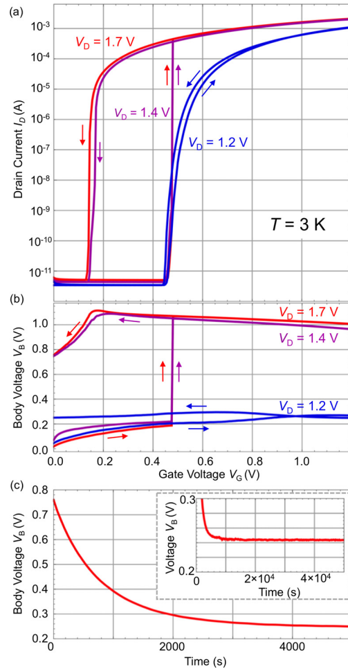
FIG. 3. (a) NMOS I_D(V_G) for V_D = 1.2, 1.4 , and 1.7 V at T \approx 3 K with substrate connected to the electrometer (no I_B due to > 10^{14} \Omega input impedance); (b) corresponding V_B(V_G) showing the complex evolution of the body potential, note that for large V_D , V_B remains finite as V_G is swept down to zero; (c) evolution of V_B after the body is charged, with the device maintained at V_G = 0 and V_D = 1.7 V, at T \approx 3 K. The decay of V_B is exponential with a time constant of 795 s. Inset shows the longer-term behavior of V_B out to 5 \times 10^4 s.
