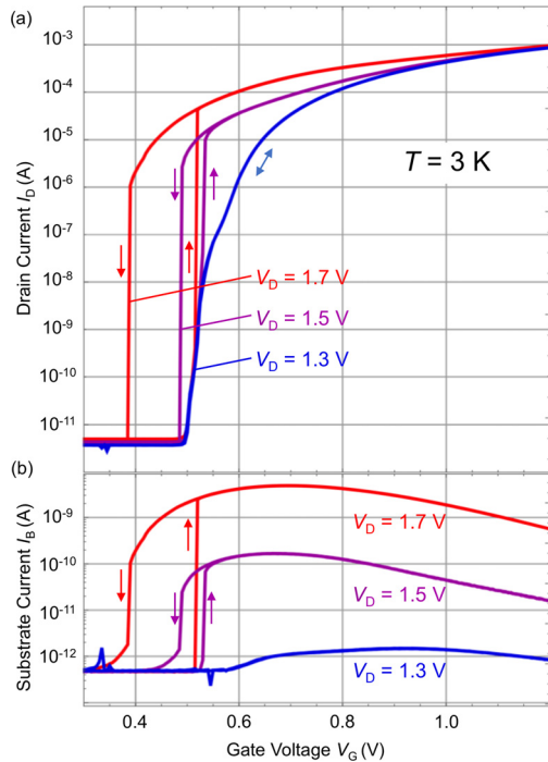
FIG. 2. (a) NMOS I_D(V_G) for V_D = 1.3, 1.5 , and 1.7 V at T \approx 3 K and V_B = 0 , showing current jumps and hysteresis developing for V_D > 1.3 V; (b) corresponding I_B for V_D = 1.3, 1.5 , and 1.7 V, measured by using the SMU substrate contact. Note that even at V_D = 1.7 V, impact ionization I_B remains < 10 nA.
