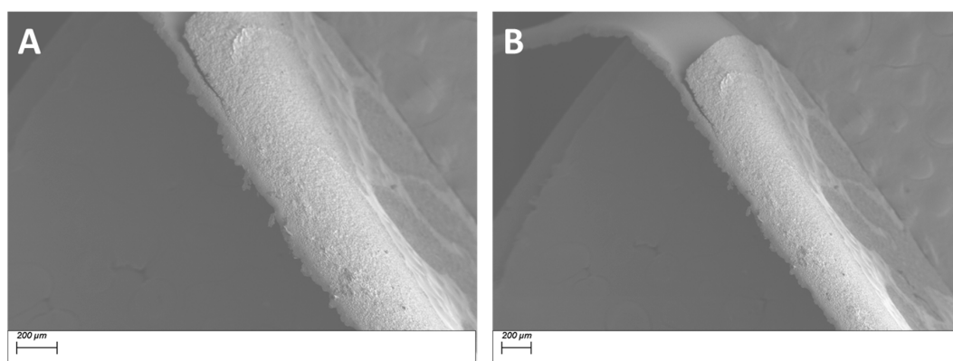
Figure 13. SEM micrograph images of the cross-section of the fractured surface of the composite that was prepared using 0.5 volume fraction 0.020 silane coupling agent BaTiO 3 nanoparticles at (A) 129 X and (B) 93 X.
