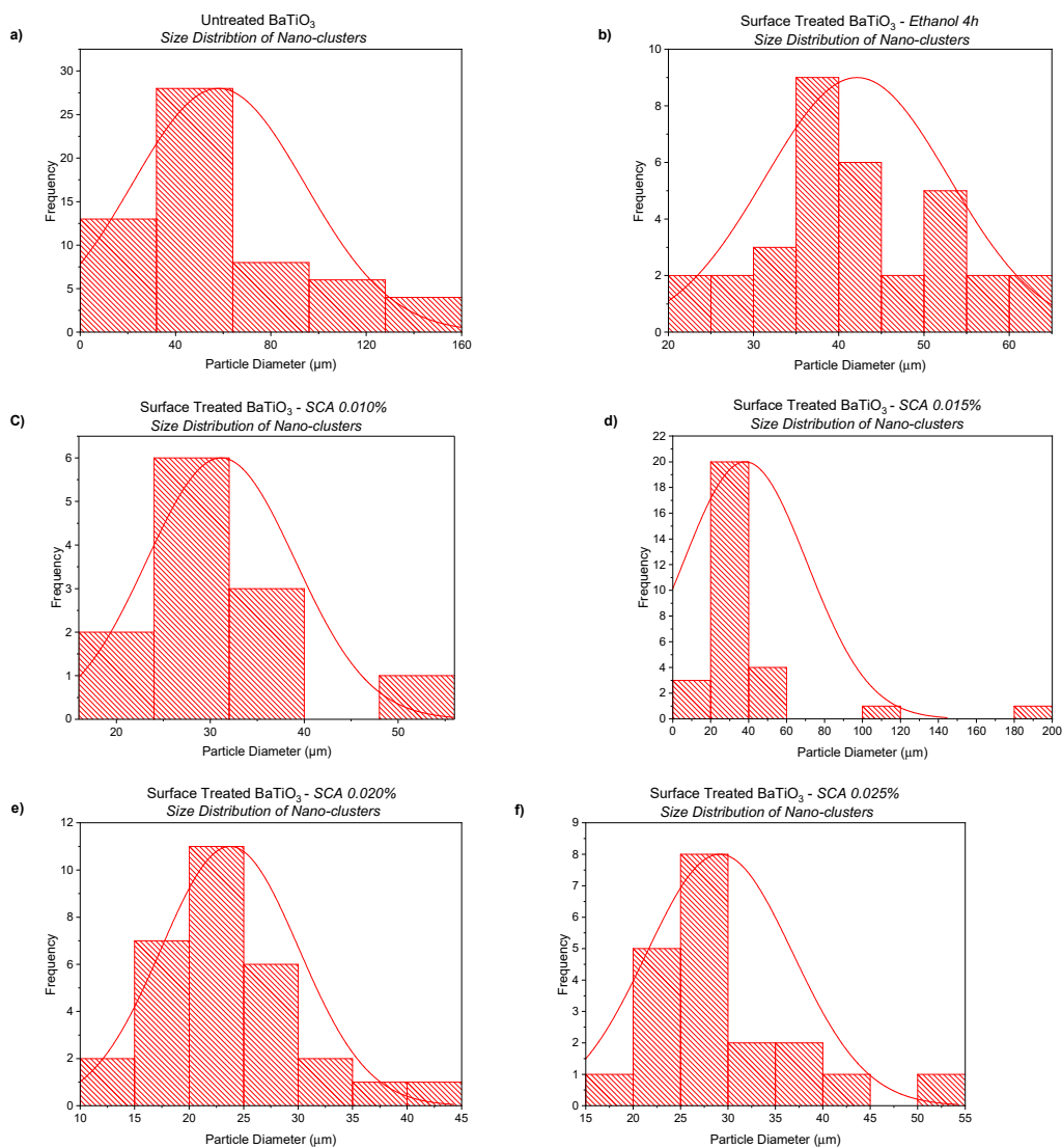
Figure 7. Particle distributions of (a) pristine BaTiO 3 which shows an average cluster size of ~60 µm, (b) ethanol surface treated for 4 h with an average cluster size of ~40 µm, (c) 0.01 silane coupling agent
