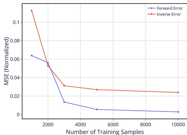
Fig. 10 Variation of INN testing accuracy with the size of the training data set
