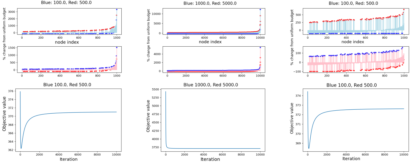
Figure 1: Top plots show percent change (from uniform strategy) of budgets at equilibrium; nodes are sorted by their component of the second eigenvector of the adjacency matrix, reflecting graph structure. The bottom panel illustrates the convergence rate of the equilibrium computation algorithm. Red and blue nodes are highlighted with dots. From left to right: a Barabasi-Albert graph of 1000 nodes and degree parameter 3, a Barabasi-Albert graph with 10000 nodes and degree parameter 3, and a Watts-Strogatz graph with 1000 nodes, initial degree 3, and rewiring probability 0.2.
