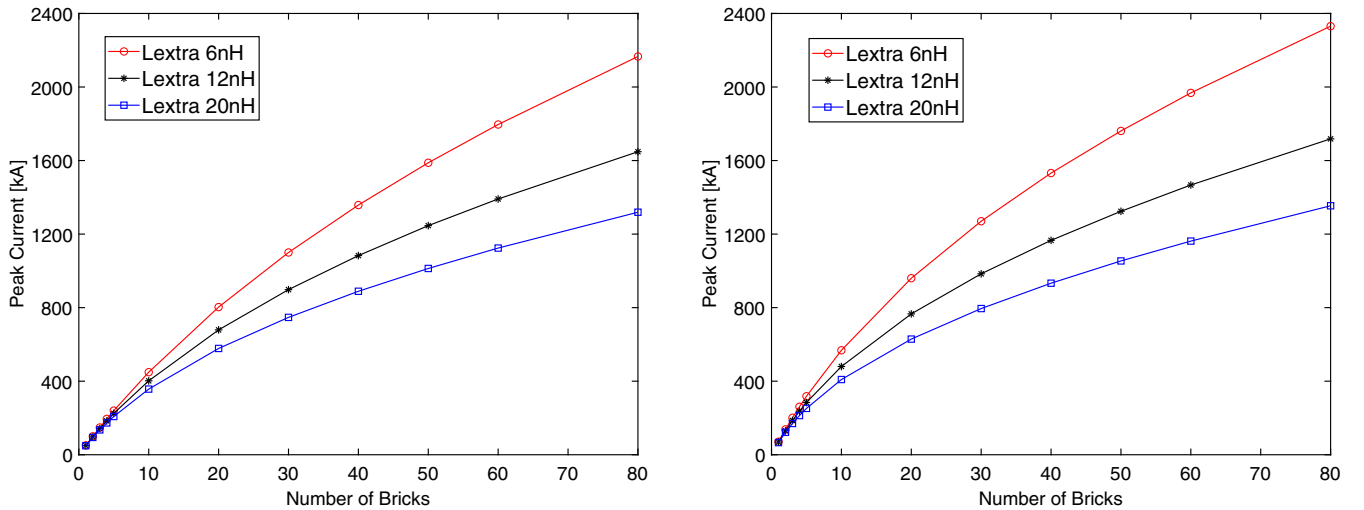
FIG. 6. Scaling of I_{\text{peak}} with N for the standard brick configuration (left) and the dry brick configuration (right) and for cases with L_{\text{extra}} = 6, 12 , and 20 nH. The load is always matched.
