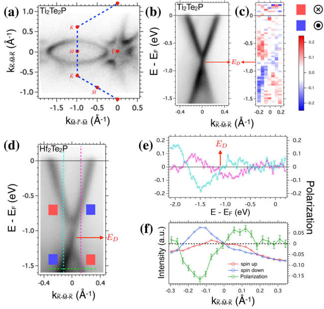
FIG. 2. (a) In-plane Fermi surface map of \text{Ti}_2\text{Te}_2\text{P} showing a sixfold symmetry. (b),(c) Near- E_F band structure of \text{Ti}_2\text{Te}_2\text{P} along the \bar{\text{K}}\bar{\text{M}}\bar{\text{K}} high-symmetry line with spin-integrated, (b), and spin-resolved, (c), ARPES, showing a Dirac-like dispersion with clear spin polarization. The color scale in (c) represents the sign and value of the in-plane spin polarization along \bar{\Gamma}\bar{\text{M}} with blue (red) pointing toward (away from) the reader. (d) Near- E_F band structure of \text{Hf}_2\text{Te}_2\text{P} along the \bar{\text{K}}\bar{\text{M}}\bar{\text{K}} high-symmetry line. Blue (red) squares indicate branches of the Dirac cone with spin polarization pointing toward (away from) the reader. (e) Energy dependent spin polarization of \text{Hf}_2\text{Te}_2\text{P} at the constant momenta indicated by the vertical light blue and magenta dashed lines in (c). (f) Spin-resolved momentum distribution curves (blue, red) and momentum dependent spin polarization (green) at the constant energy indicated by the horizontal green dashed line in (d). Spin up and spin down means parallel and antiparallel to \bar{\Gamma}\bar{\text{M}} . The Dirac point at energy E_D is shown by a red arrow in panels (b)–(e). All data were collected with LH polarized photons of 55 eV. The temperature was 25 K.
