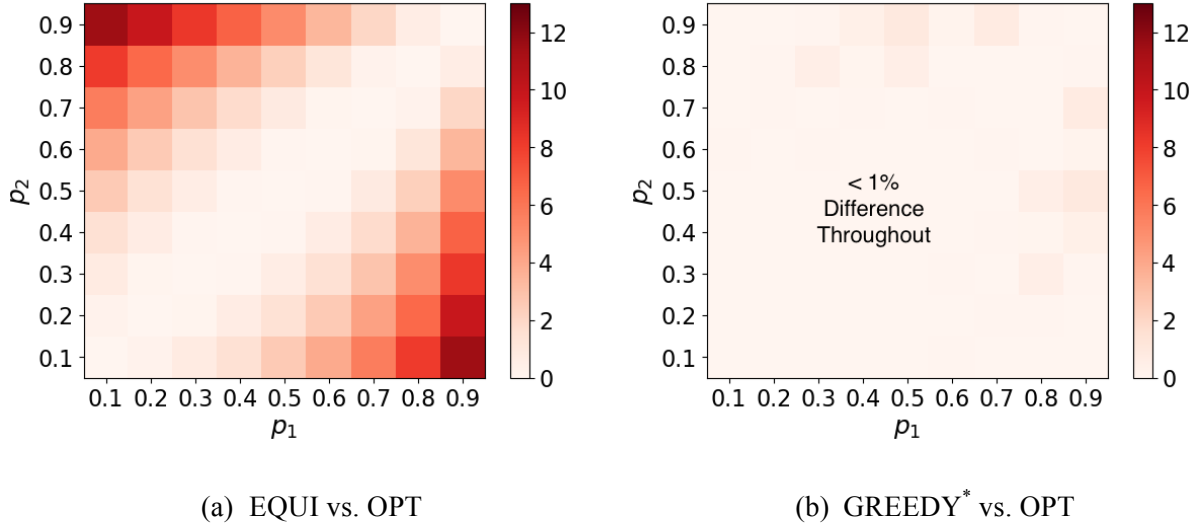
Figure 3. Heat maps showing the percentage difference in mean response time, \mathbb{E}[T] , between (a) EQUI and OPT and between (b) GREEDY* and OPT , in the case of two speedup functions where s_1 and s_2 are Amdahl's law with parameters p_1 and p_2 respectively. Here \mathbb{E}[X] = \frac{1}{2} and \Lambda_1 = \Lambda_2 = 5 . The axes represent different values of p_1 and p_2 . GREEDY* , EQUI , and OPT were evaluated numerically using the MDP formulation given in Section 4.5. These heat maps look similar under various values of \Lambda_1 and \Lambda_2 .
