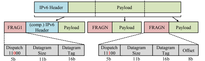
Fig. 7: Packet Fragmentation.
