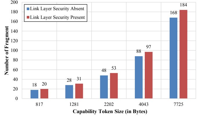
(b) Token size Vs. Packet fragments (Route-over routing).
