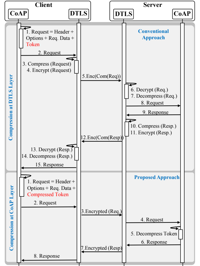
Fig. 14: The operational model of token compression procedure.
