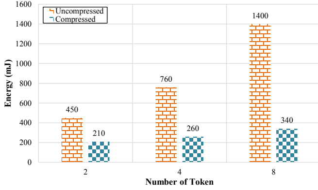
(a) Communication energy consumption for authorization tokens.
