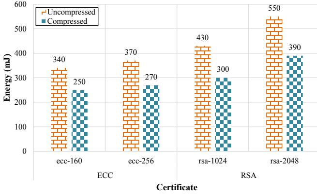
(b) Communication energy consumption for certificates.
