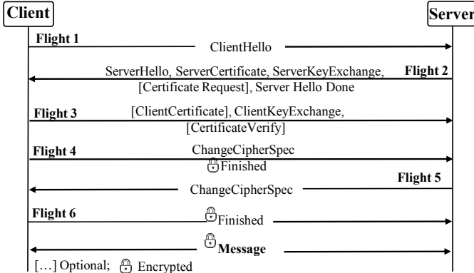
Fig. 5: A fully authenticated DTLS handshake.
