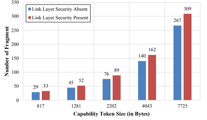
(a) Certificate size Vs. Packet fragments (Mesh-under routing).
