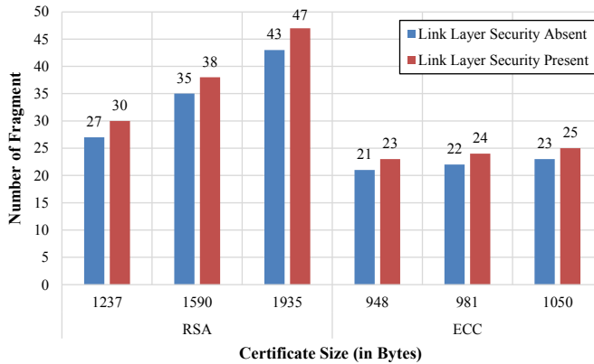
(b) Token size Vs. Packet fragments (Route-over routing).
