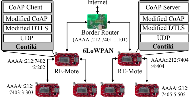
Fig. 15: Experimental setup. Modified CoAP = CoAP + CapBAC Token Compression. Modified DTLS = DTLS + Certificate Compression.
