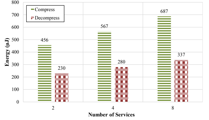
(a) CPU energy consumption to compress and decompress the tokens.
