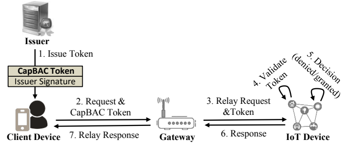
Fig. 2: The CapBAC model.
