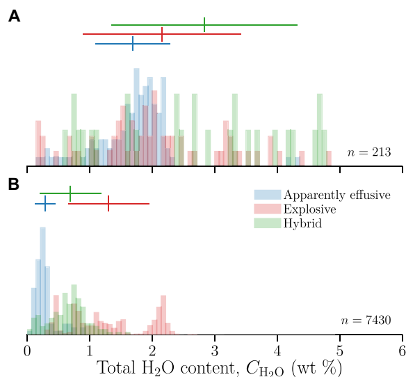
Fig. 1. The water content of erupted rhyolites worldwide. (A) The distribution of dissolved water measured in glass inclusions trapped in crystals for a range of rhyolite eruptions (213 data points) (10–12). Taken to represent the initial, dominant volatile conditions for ascent, these values are similar in variance and mean value and do not vary substantially with eruptive style (we do not account for volatile loss after entrapment). (B) The distribution of dissolved total water content remaining in the groundmass glass of eruptive products, in a second global database of rhyolite compositions compiled here (7430 data points) (10, 12–19, 46). Effusive eruption products have substantially lower water than explosive products; hybrid products fill the gap, forming a continuum. wt % is used to denote weight %.
