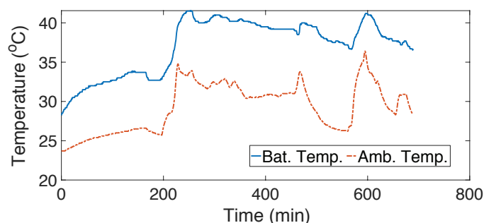
FIGURE 3. The temperature of a mobile device's battery is strongly correlated with that of its ambient environment.
