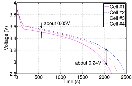
Fig. 5. The voltage traces of four cells in a battery pack, demonstrating clear heterogeneity.
