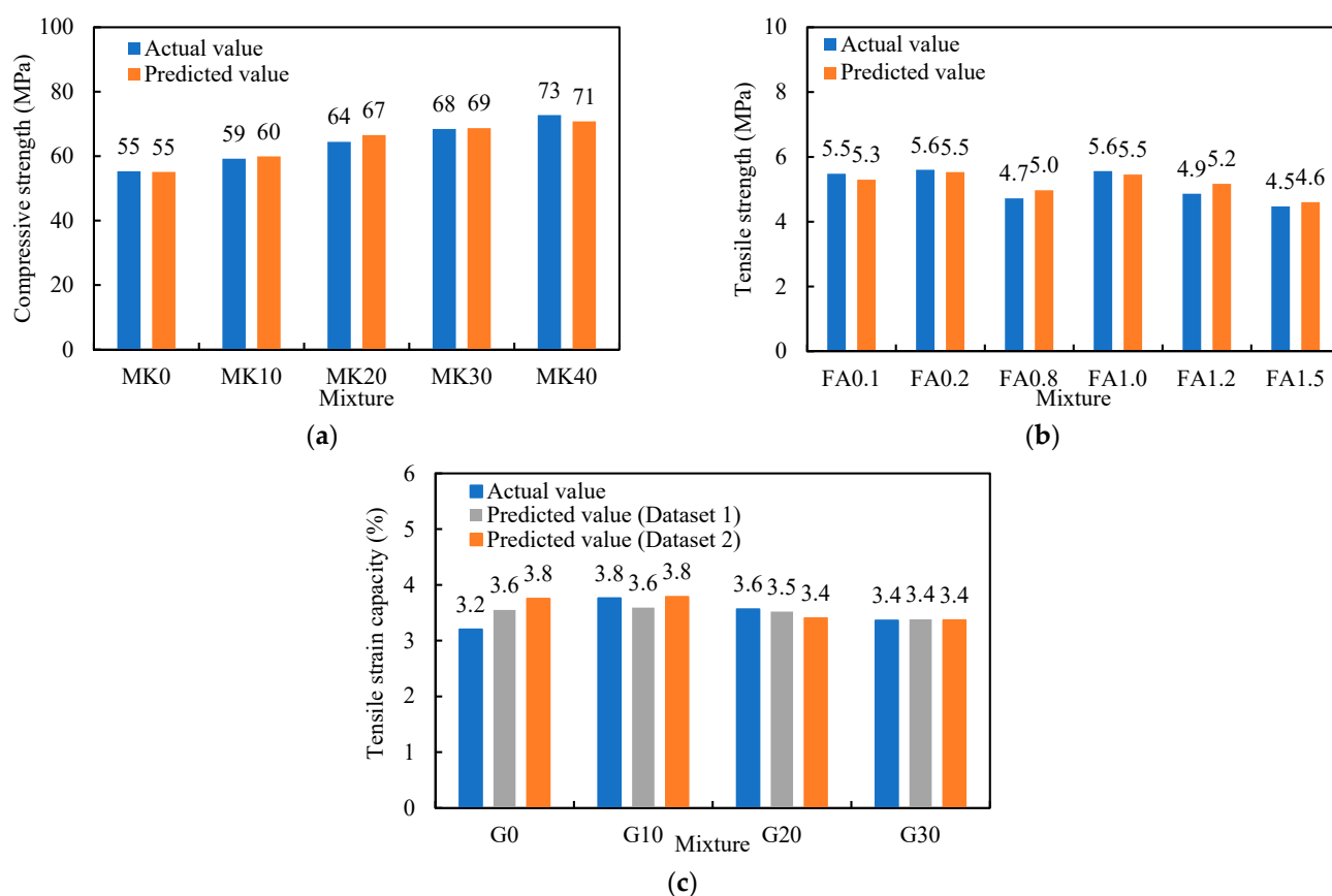
Figure 9. Comparison of the prediction against the test results: (a) compressive strength [77]; (b) tensile strength [22]; and (c) tensile strain capacity [63].
