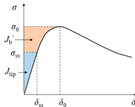
Figure 3. Illustration of the stress-crack opening curve for HPFRCC. The orange area represents the complementary energy ( J_b' ), and the blue area represents the crack tip toughness ( J_{tip} ).
