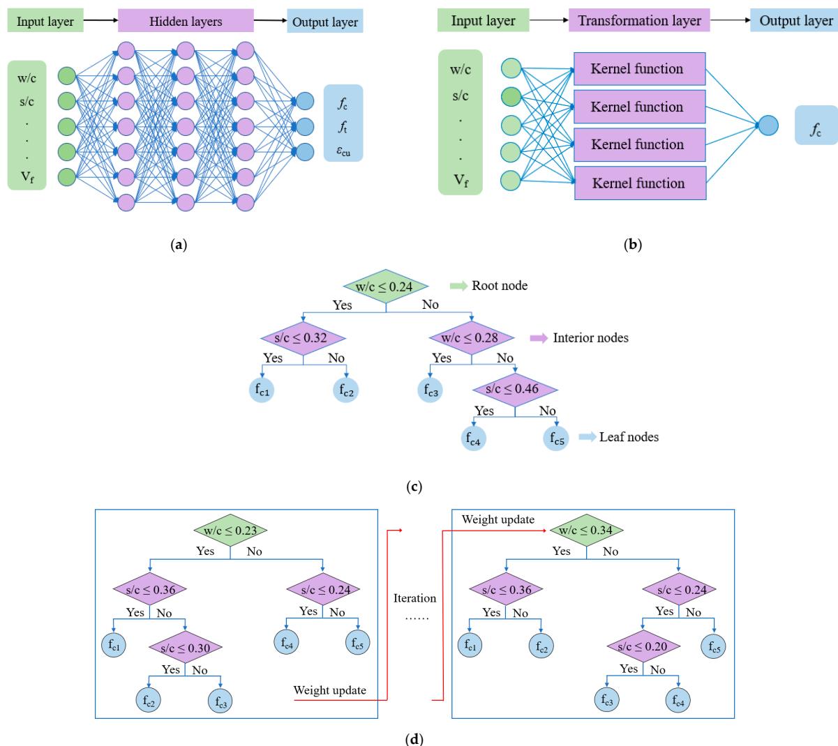
Figure 1. Machine learning models: (a) ANN; (b) SVR; (c) CART; and (d) XGBoost. w/c is the water-to-cement ratio; s/c is the sand-to-cement ratio; V f is the fiber content; f c is the compressive strength; f t is the tensile strength; and ε cu is the tensile strain capacity (i.e., ductility).
