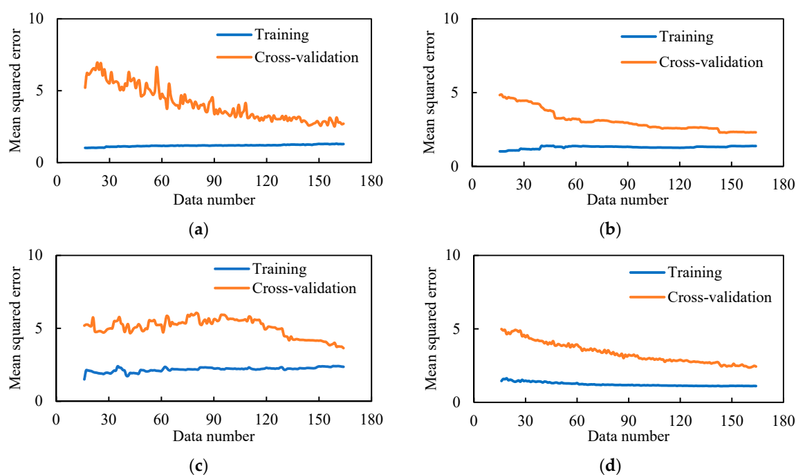
Figure 7. Learning curve for the training process (tensile strength) using: (a) ANN, (b) SVR, (c) CART, and (d) XGBoost.
