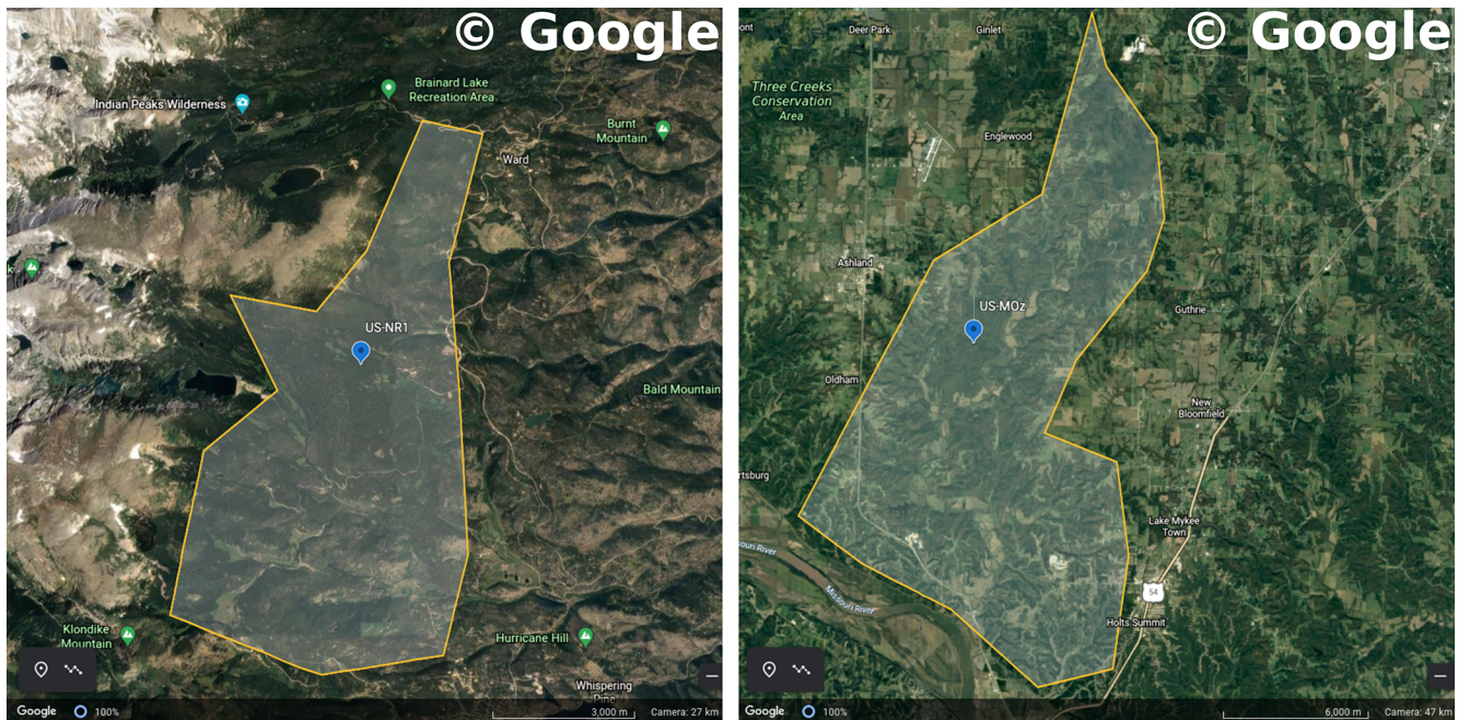
Figure 7. Regions chosen to filter TROPOMI SIF observations. The left panel shows a Google Earth map for the US-NR1 flux tower site (Niwot Ridge, Colorado, USA). The right panel shows a Google Earth map for the US-MOz flux tower site (Ozark, Missouri, USA). The blue symbols show the flux tower locations, and the shaded regions are representative of area around the flux tower site. Map data were sourced from ©Google Earth Landsat/Copernicus.
