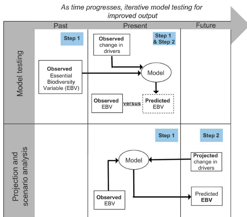
Figure 6. Framing of the multivariate approach to evaluating and reducing uncertainty in model-based biodiversity projections within a broader model testing, biodiversity policy, and decision-making context. The approach to constrain biodiversity uncertainty via both univariate (step 1 from figure 1) and multivariate constraints (step 2 from figure 1) are mapped in the present article to show at what time step (past, present, or future) remote sensing, in-situ observations, and multimodel overlap of related biodiversity variables can directly constrain initial conditions of an EBV (past), directly and indirectly constrain EBV uncertainty to improve and refine model output (present), and indirectly constrain uncertainty of EBV projections (future).
