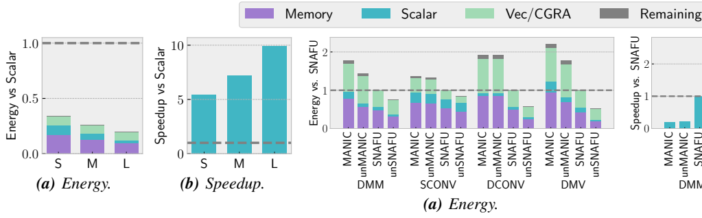
Figure 9: SNAFU-ARCH vs. the scalar design across three input sizes – small (S), medium (M) and large (L).
