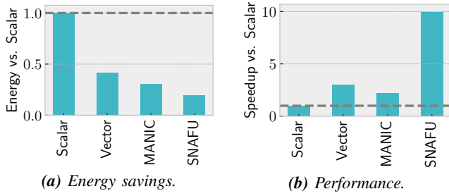
Figure 1: SNAFU-ARCH’s energy and performance normalized to a scalar baseline. On average, SNAFU uses 81% less energy and is 9.9 \times faster, or 41% less energy and 4.4 \times faster than MANIC.
