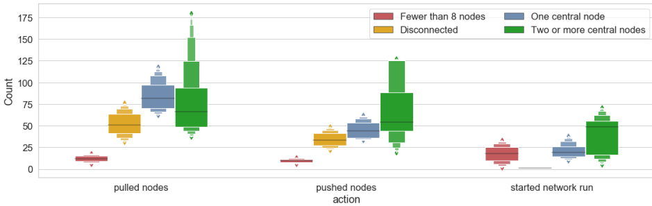
Fig. 16. Frequency of collaborative tasks performed in MIDST
