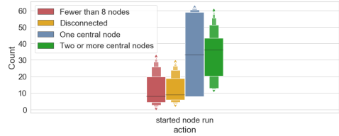
Fig. 18. Running nodes assigned to other team members
