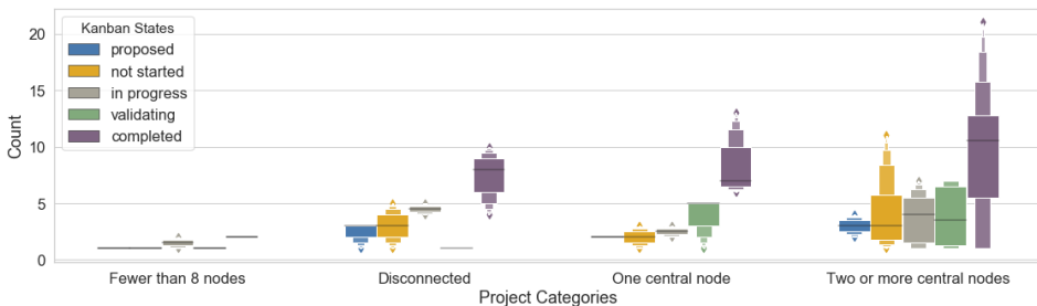
Fig. 14. Usage of node kanban stage by complexity of workflow
