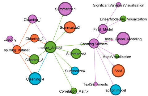
Fig. 13. A workflow with two or more nodes with high betweenness
