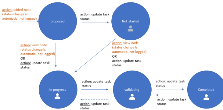
Fig. 3. Transitions of node status
