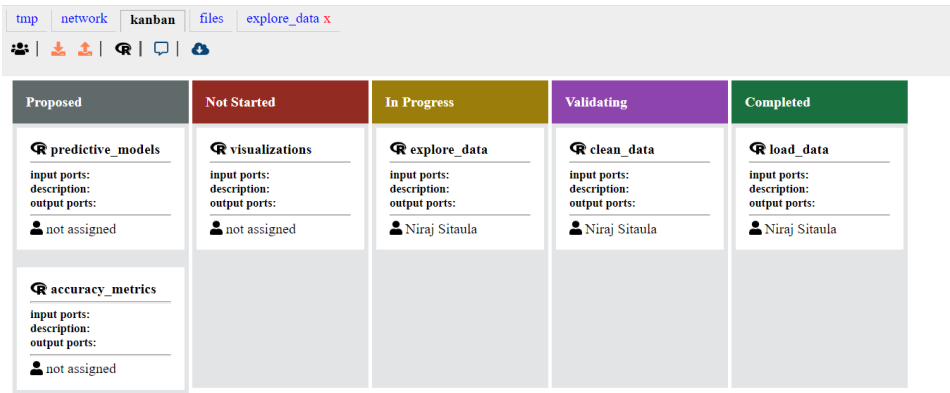
Fig. 4. Kanban view in MIDST
