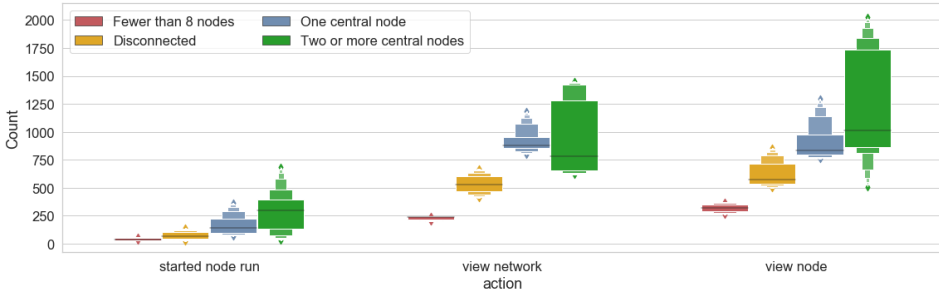
Fig. 15. Frequency of individual tasks performed in MIDST
