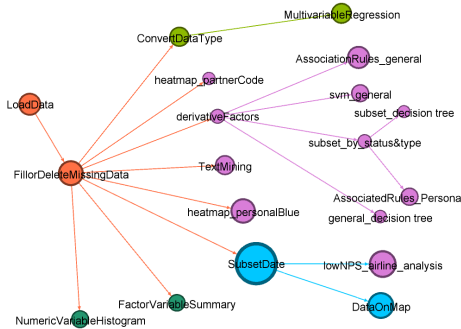
Fig. 12. A workflow with two or more nodes with high betweenness
